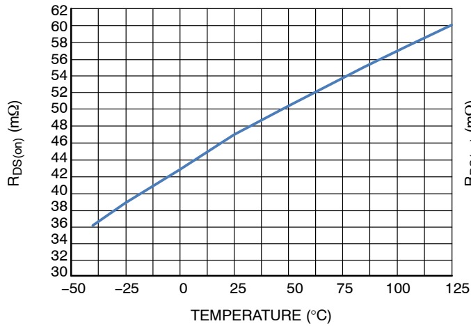
Figure 6. R_{DS(on)} ( m\Omega ) vs. Temperature (°C) at 3.3 V, I_{load} 100 mA
