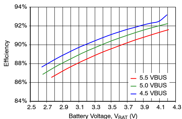
Figure 9. Charger Efficiency vs. V_{BUS} , I_{INLIM} = 500\text{ mA}
