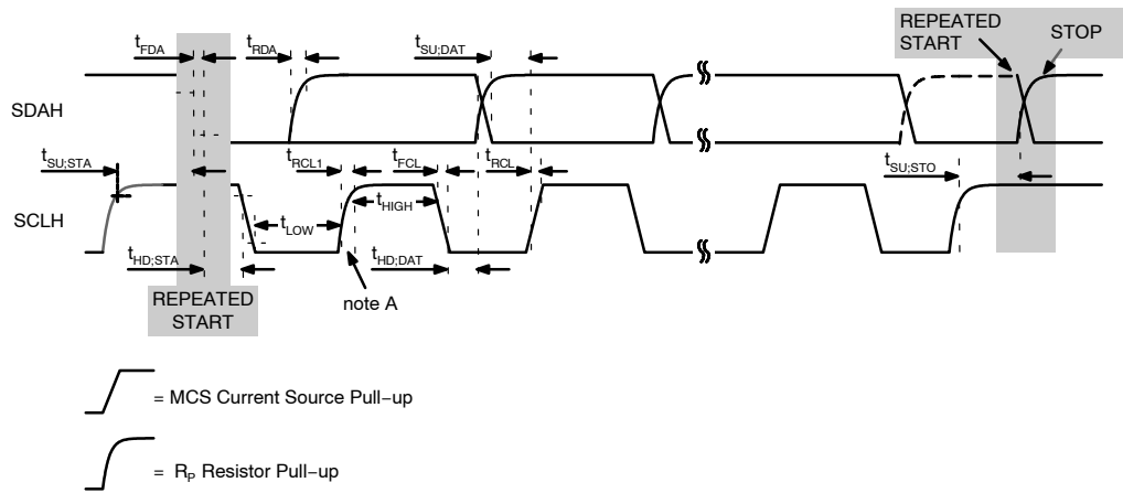
Figure 5. I²C Interface Timing for High-Speed Mode
