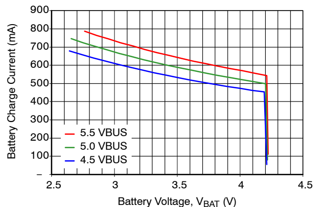
Figure 7. Battery Charge Current vs. V_{BUS} with I_{INLIM} = 500\text{ mA}
