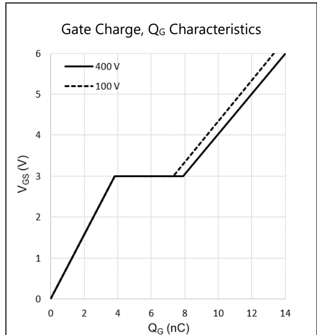
Figure 6: Typical V_{GS} vs. Q_G @ V_{DS} = 100, 400V
