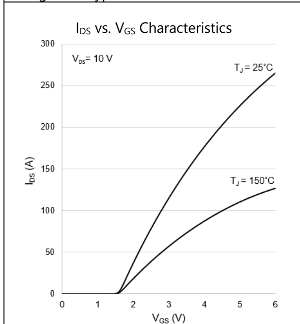
Figure 11: Typical I_{DS} vs. V_{GS}
