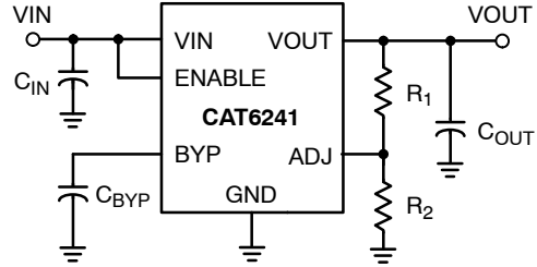
Figure 37. Adjustable Output Resistor Divider
