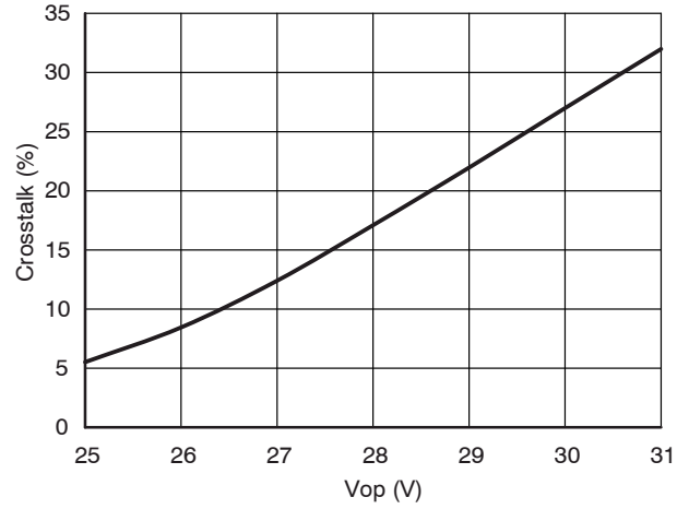
Figure 4. Crosstalk vs. Bias Voltage
