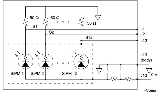
Figure 10. ArrayRDM-0112A20-GEVB Board Schematic
