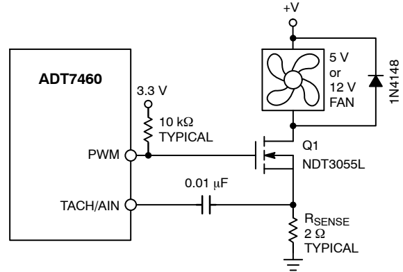
Figure 44. Driving a 2-wire Fan
