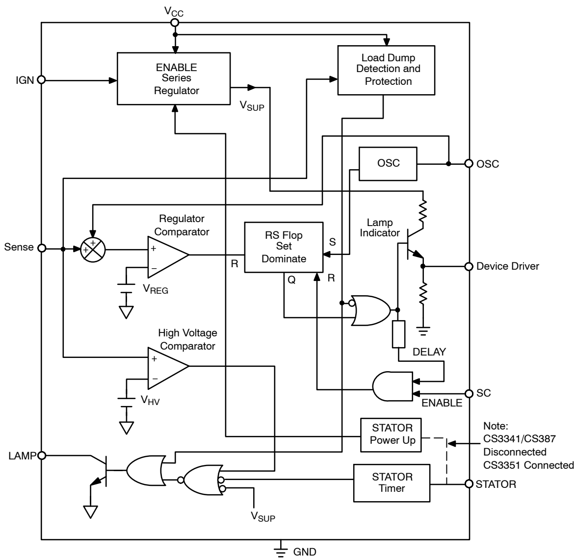
Figure 1. Block Diagram
