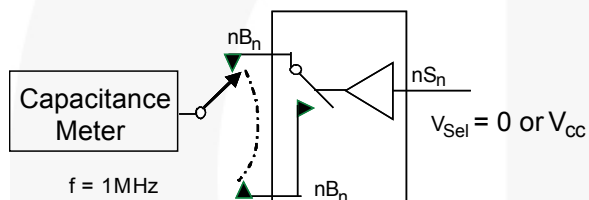
Figure 14. Channel Off Capacitance
