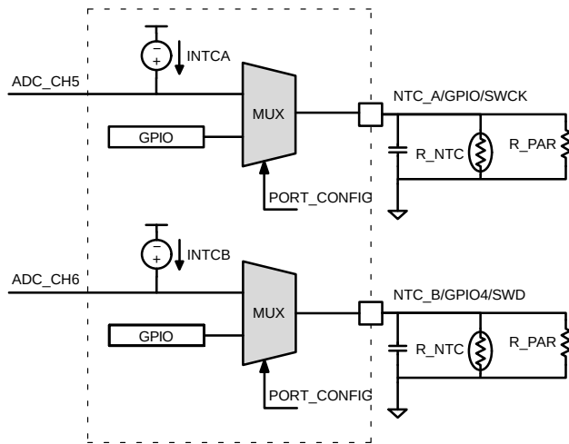
Figure 8. External Temperature Monitoring
