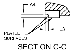
SECTION C-C
