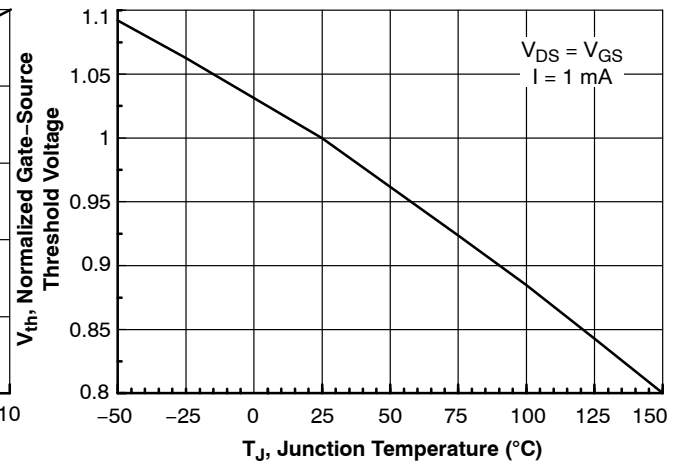
Figure 6. Gate Threshold Variation with Temperature
