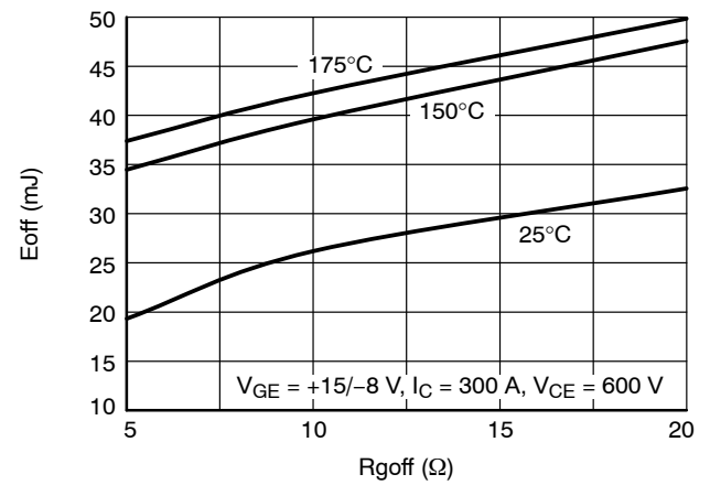
Figure 10. IGBT Turn-off Losses vs. R_{Goff}
