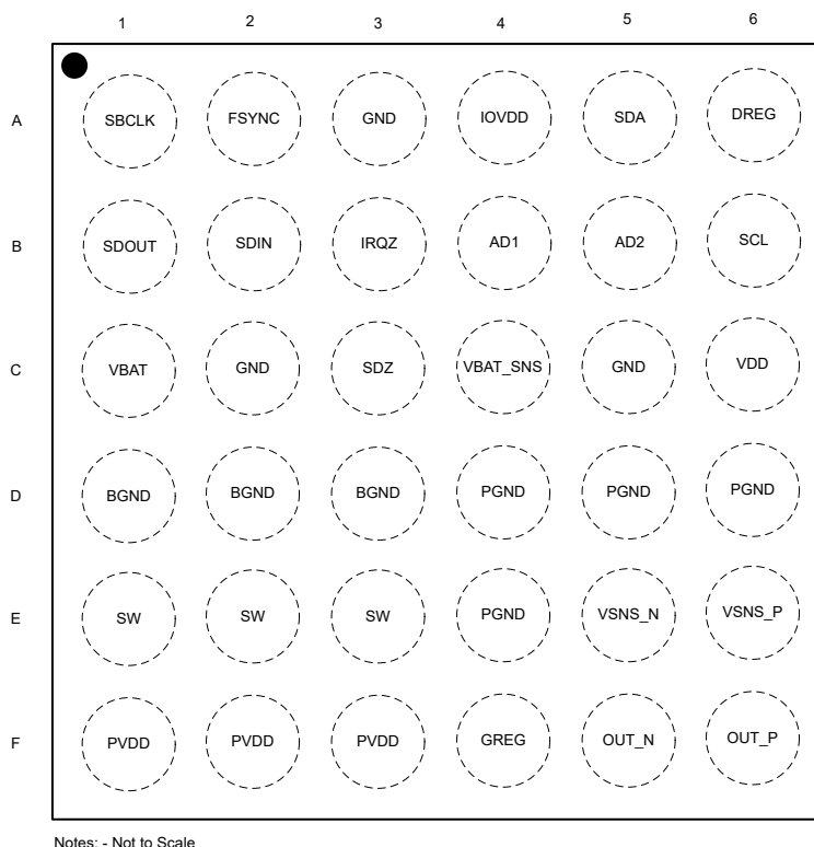
Figure 4-1. Package Top Level View Pinout
