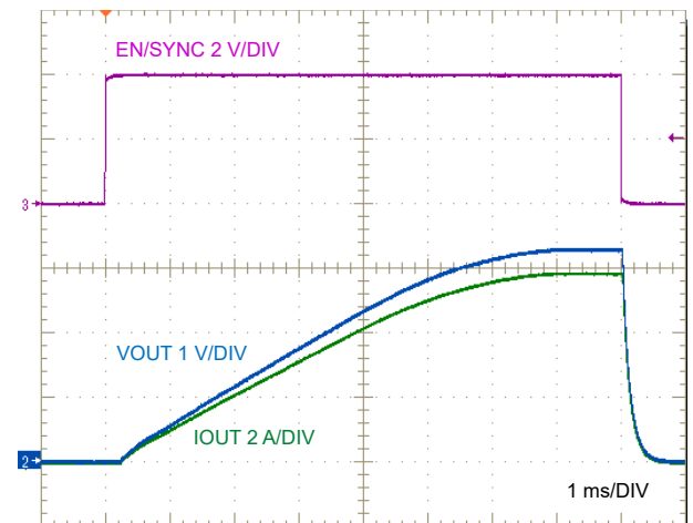
图 8-25. LM634x0-Q1 Enable On, Off, 6A Resistive Load
