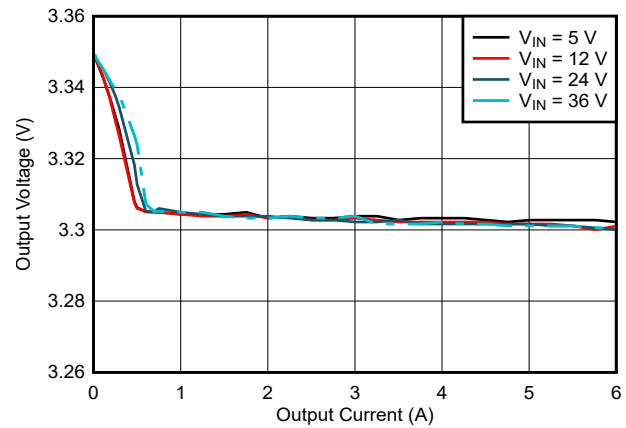
图 8-23. LM634x0-Q1 Load and Line Regulation
