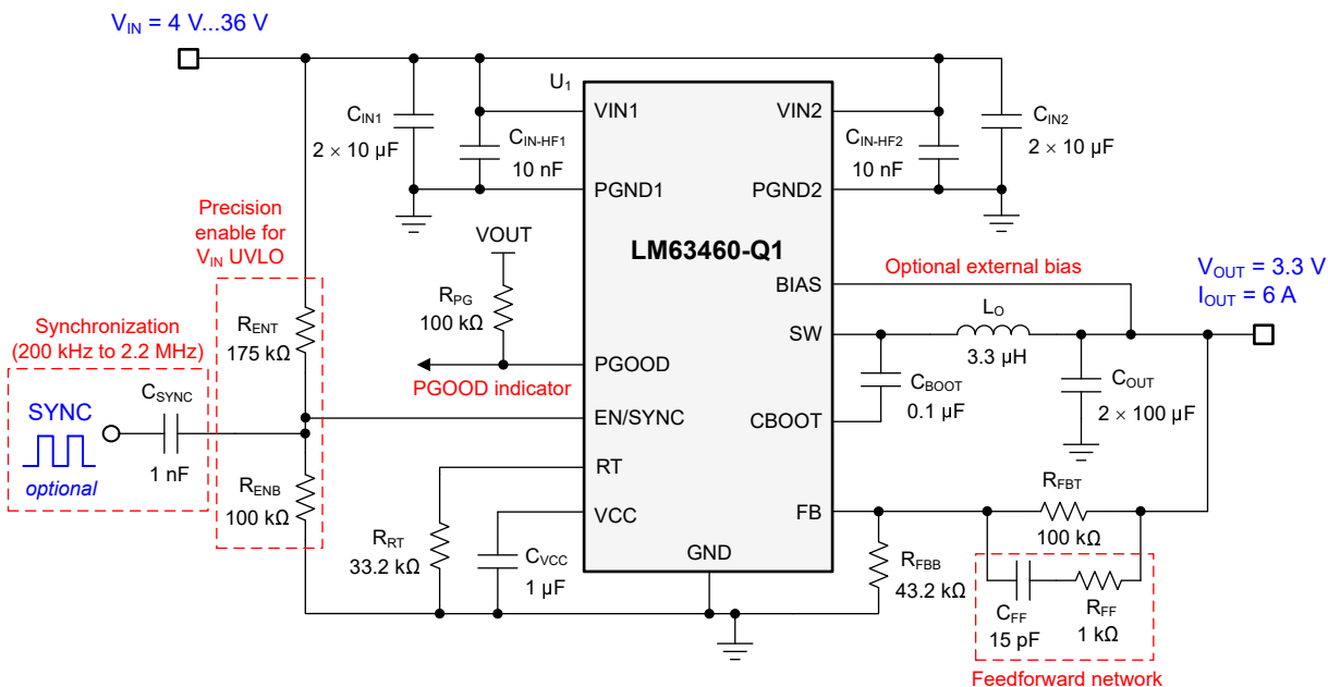
图 8-21. Application Circuit 3 – 3.3V, 6A at 400kHz
