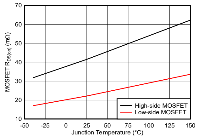
图 6-6. High-Side and Low-Side MOSFET R_{DS(on)}
