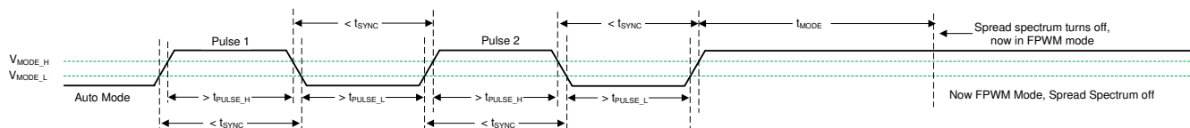
图 7-9. Spread Spectrum Disabled in Transition from AUTO Mode to FPWM Mode
