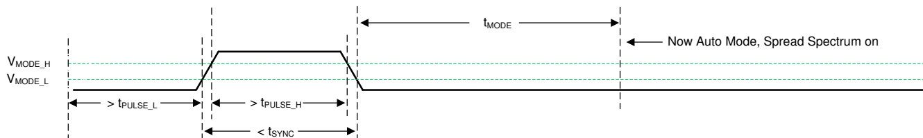
图 7-10. Transition from SYNC Mode to AUTO Mode
