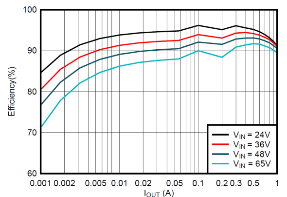
图 6-3. 5V PFM Efficiency Versus Load Current
