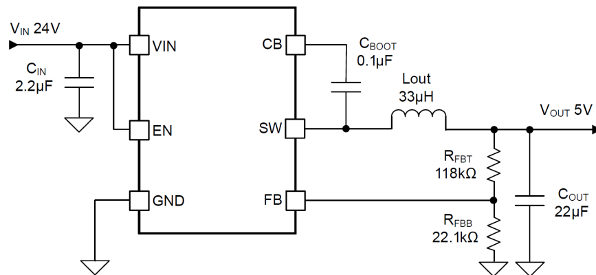
图 8-1. Application Circuit
