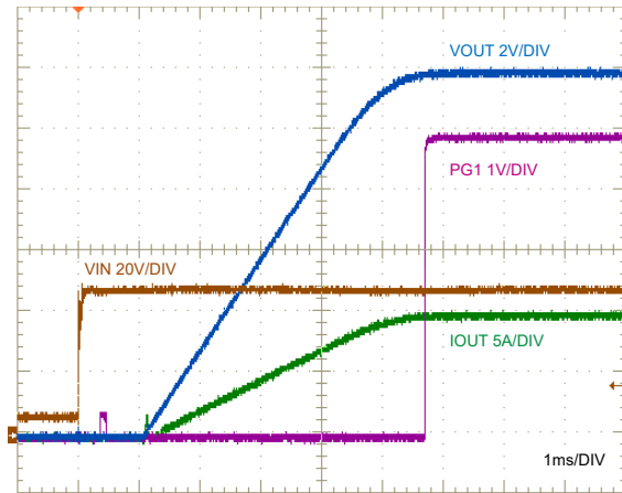
Figure 8-19. Start-Up Characteristic
