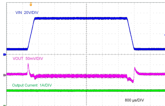
LMR38015 V_{OUT} = 5V 400kHz
