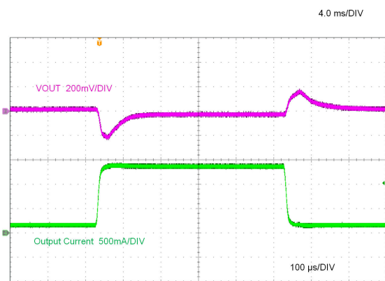
LMR38015 V_{OUT} = 5V 400kHz
