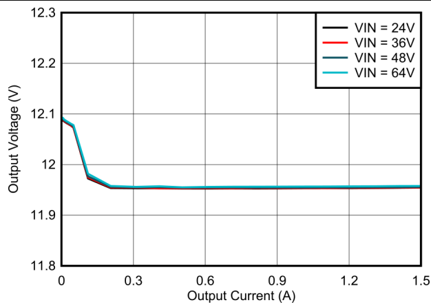
LMR38015 V_{OUT} = 12V 400kHz
