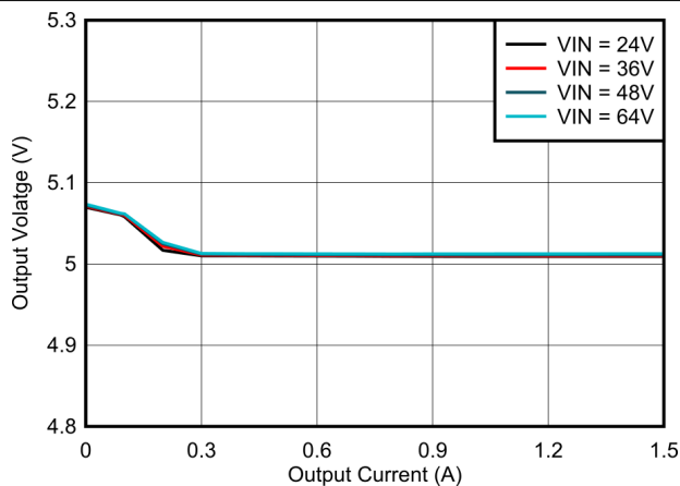
LMR38015 V_{OUT} = 5V 400kHz
