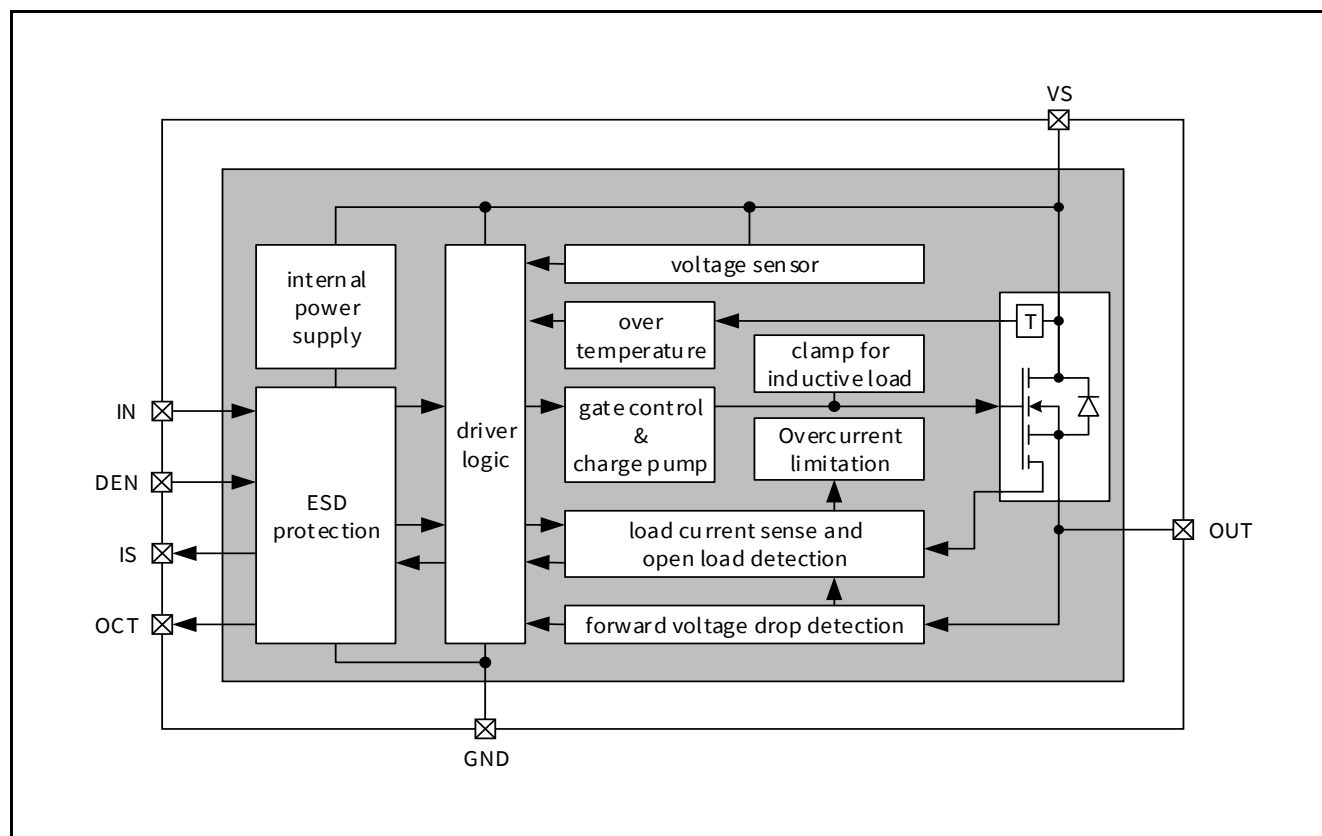
Figure 1 Block Diagram for the BTT6080-1ERL
