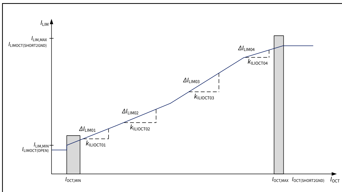
Figure 18 Adjustable overcurrent threshold behavior
