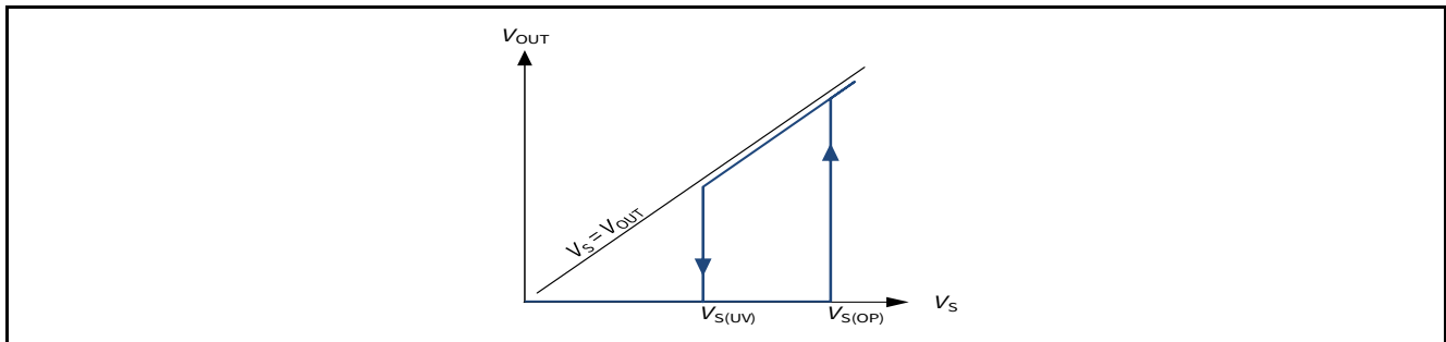
Figure 15 Undervoltage Behavior
