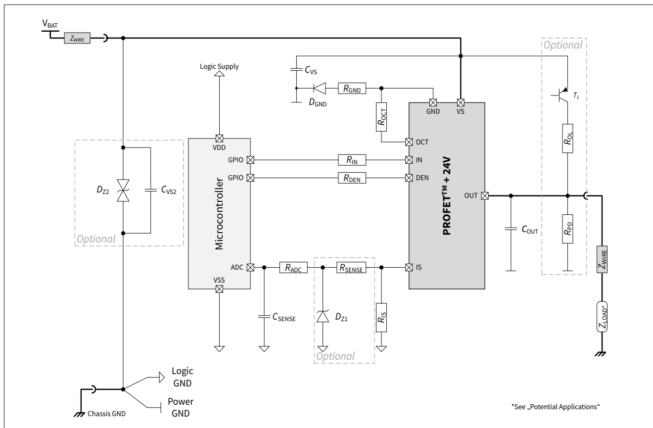
Application Diagram with BTT6080-1ERL
