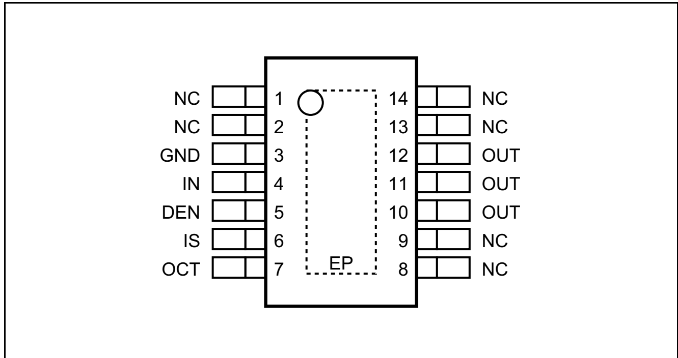
Figure 2 Pin configuration PG-TDSO-14
