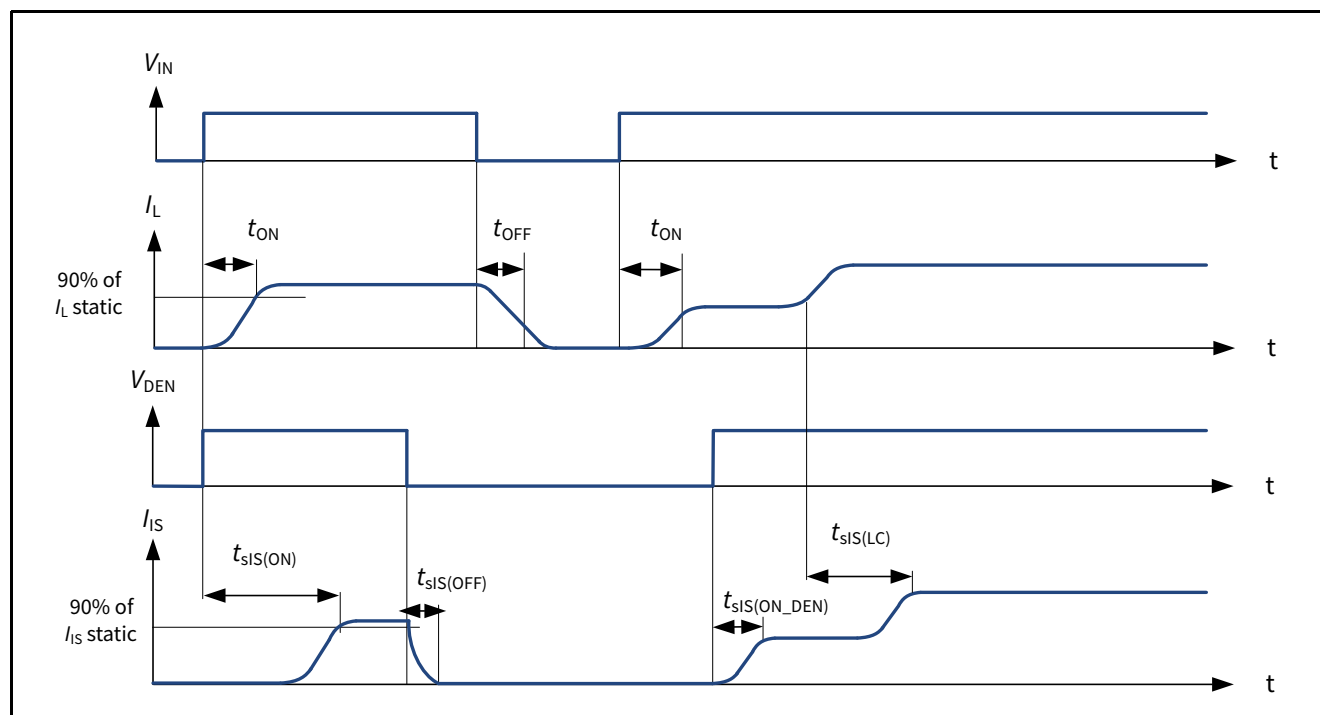
Figure 23 Current Sense Settling / Disabling Timing
