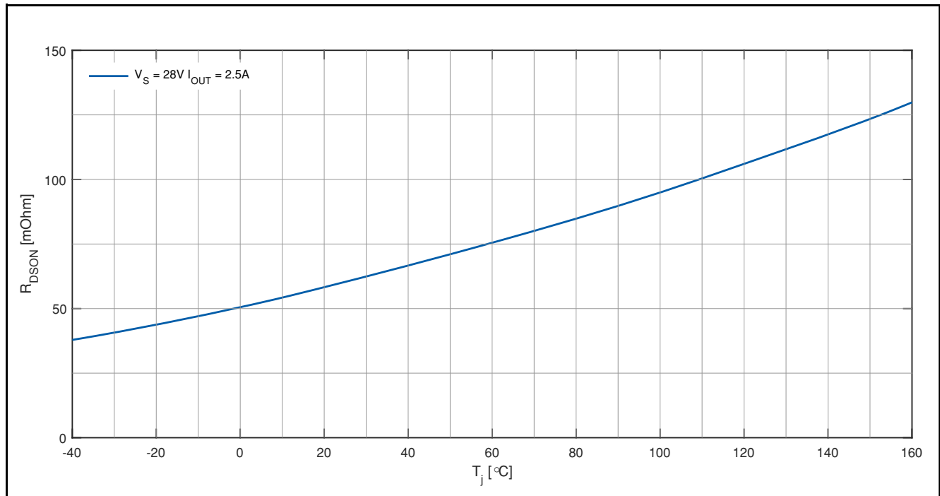
Figure 8 Typical ON-State Resistance
