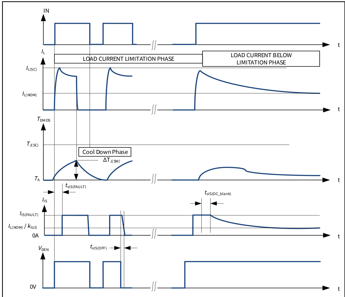
Figure 19 Overload Protection
