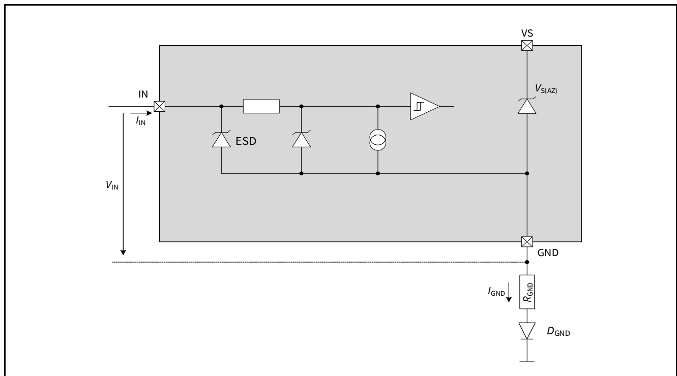
Figure 28 Input Pin Circuitry
