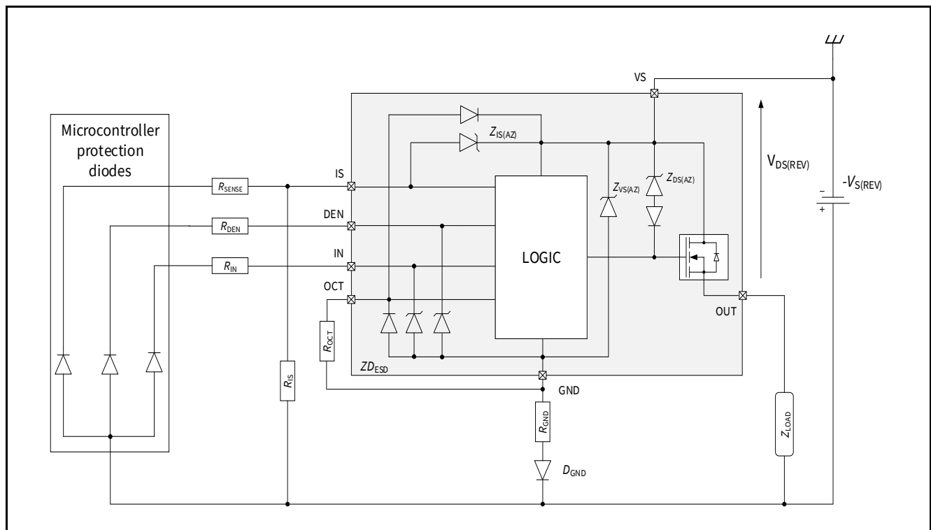
Figure 17 Reverse Polarity Protection with External Components
