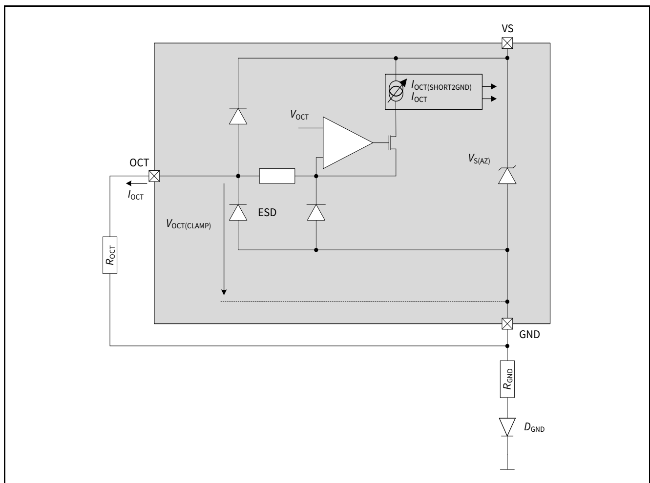
Figure 29 Overcurrent pin circuit
