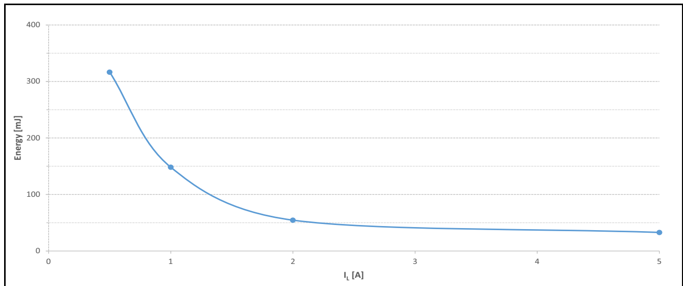
Figure 12 Maximum Energy Dissipation Single Pulse, T_{J\_START} = 150^\circ\text{C} ; V_S = 28 \text{ V}
