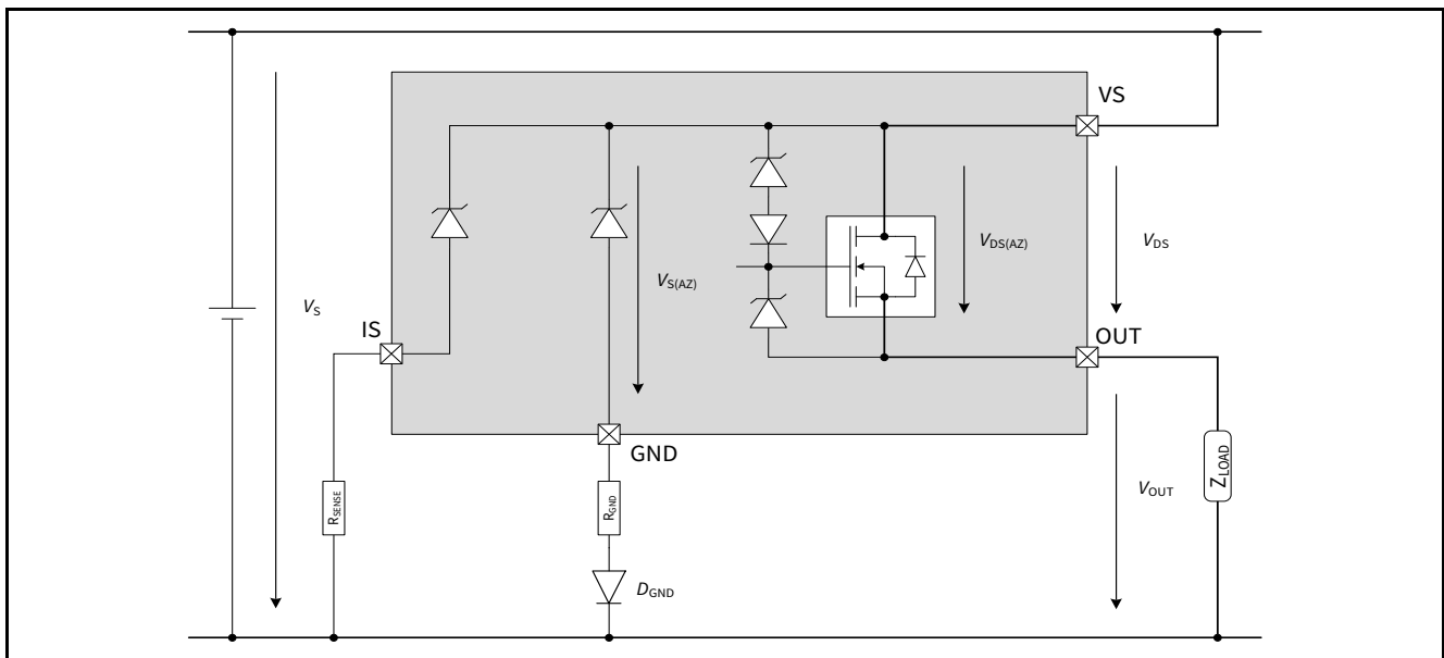
Figure 10 Output Clamp
