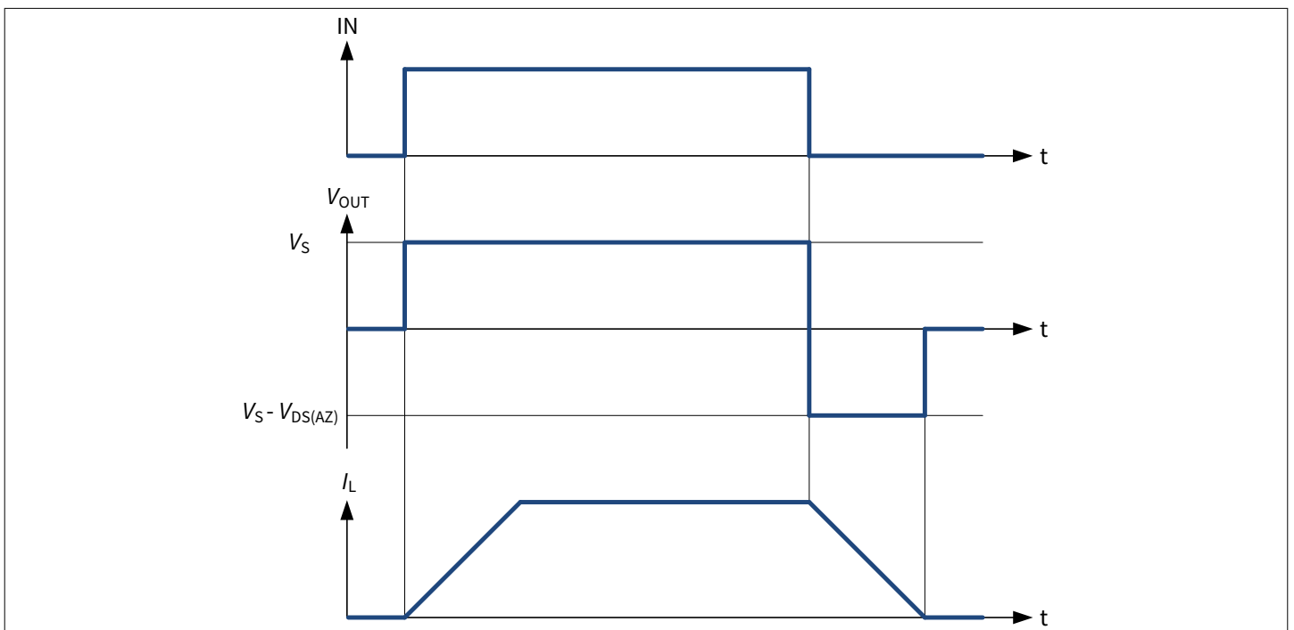
Figure 12 Switching an Inductive Load Timing
