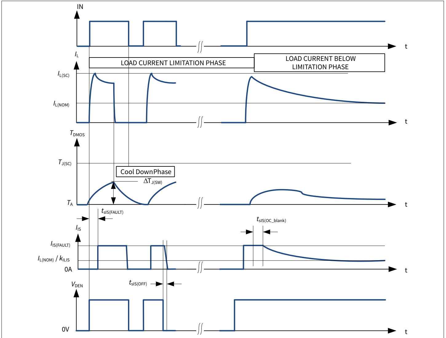
Figure 20 Overload Protection
