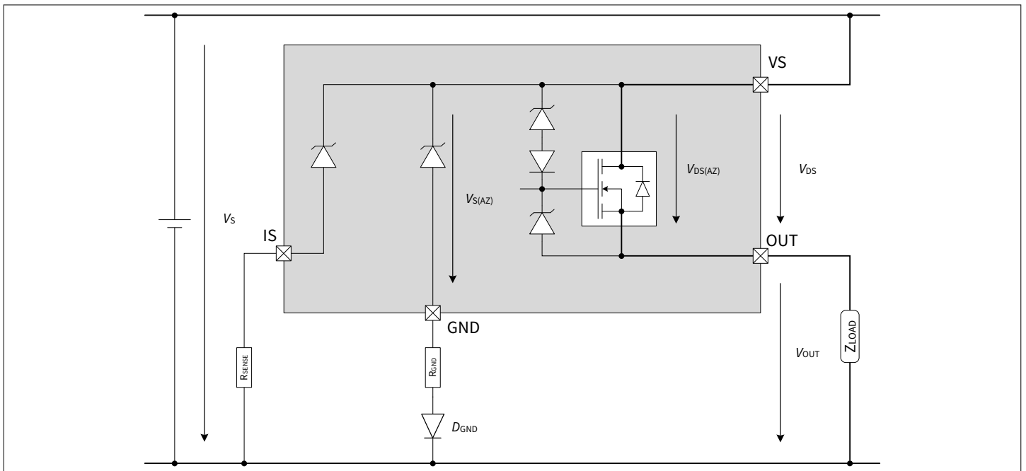
Figure 11 Output Clamp
