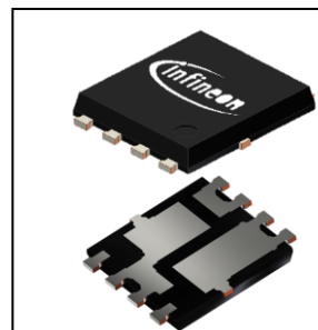
PG-TDSON-8-57
