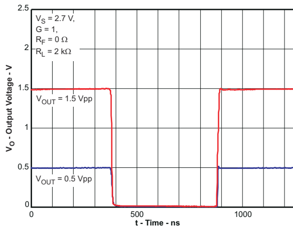
图 7-3. Noninverting Pulse Response
