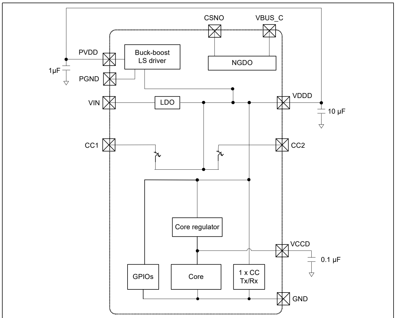
Figure 8 Power system requirement block diagram
