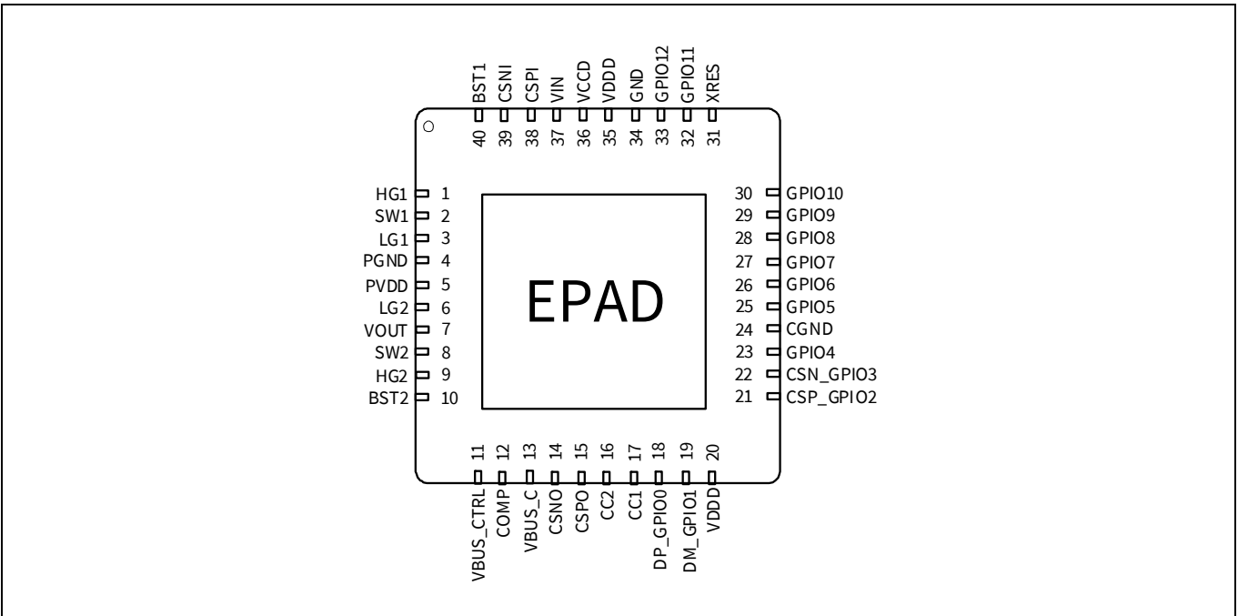
Figure 9 EZ-PD™ CCG7S 40-QFN pinout
