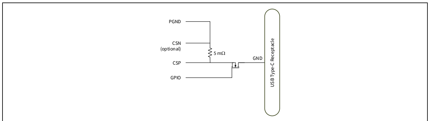
Figure 1 VBUS to ground short circuit protection
