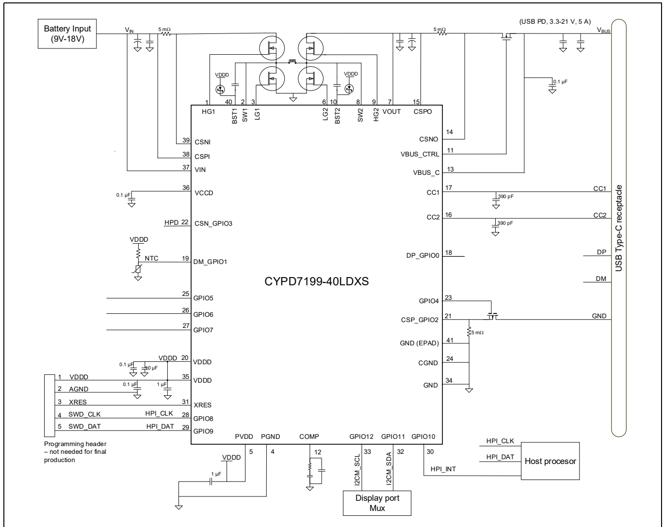
Figure 15 EZ-PD™ CCG7S rear seat entertainment (RSE) application diagram
