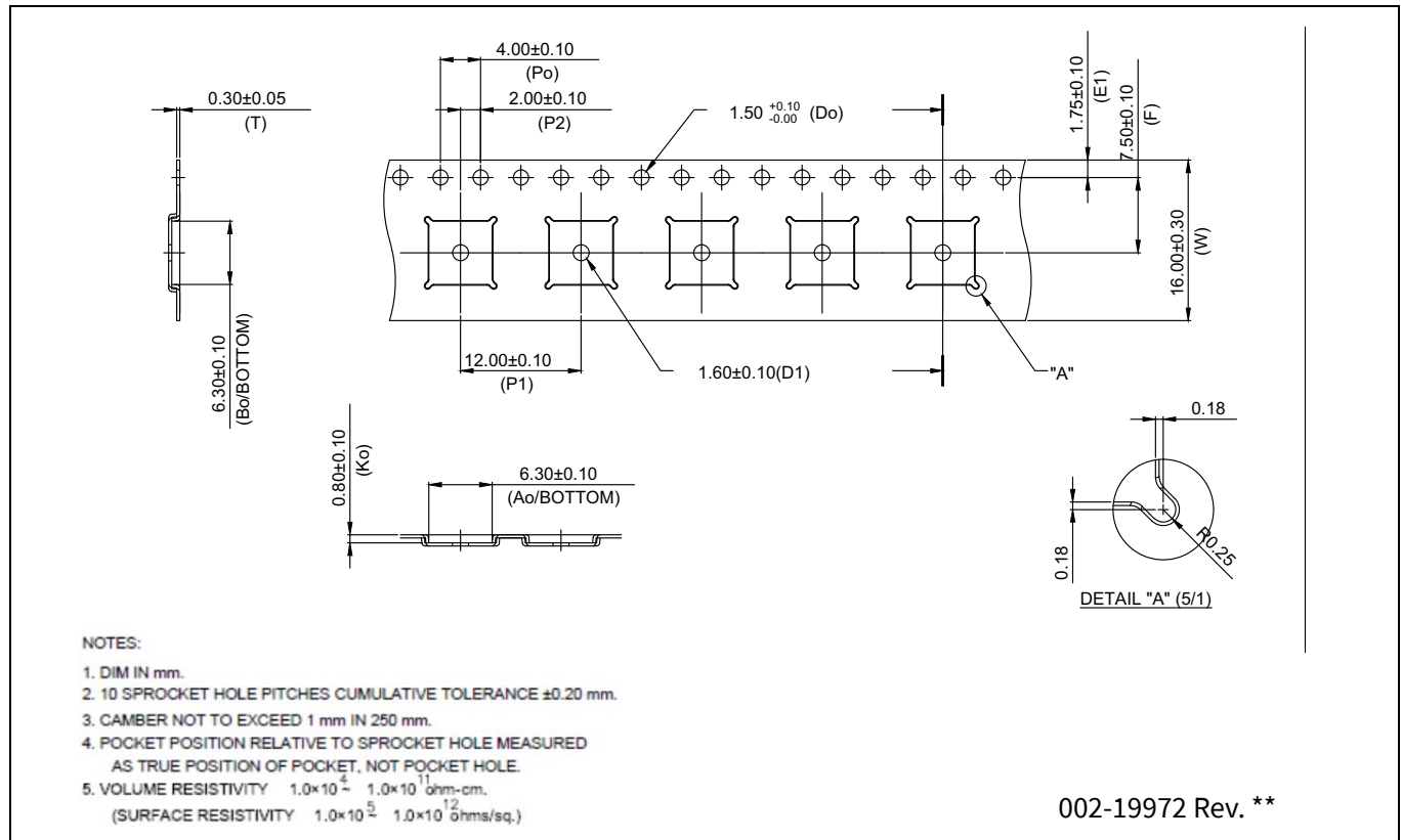
Figure 17 Carrier Tape, QFN0606 (HWA SHU), 002-19972
