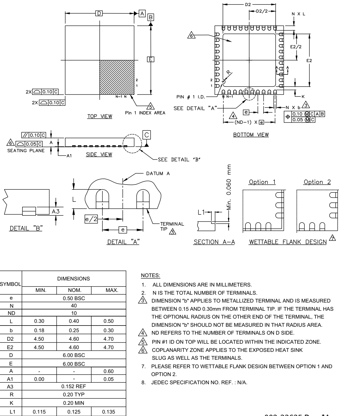
Figure 16 40 LEAD QFN ((6.0 × 6.0 × 0.6 mm) LD40D 4.60 × 4.60 mm EPAD (Wettable flank)) package outline, 002-33635
