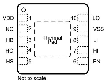
Figure 4-1. DRC Package 10-Pin SON Top View
