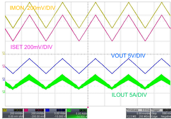
图 7-13. ISET 调制, V_{\text{SUPPLY}} = 48\text{V} , R_{\text{LOAD}} = 1.35\ \Omega
