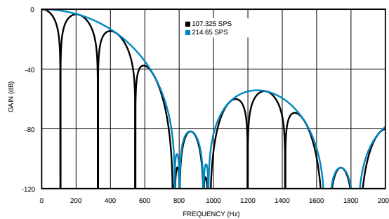
Figure 49. Digital Filter Response 107.325 SPS and 214.65 SPS
