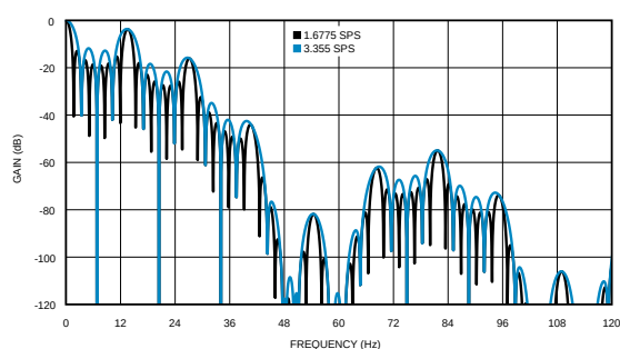
Figure 41. Digital Filter Response, 1.6775 SPS and 3.355 SPS
