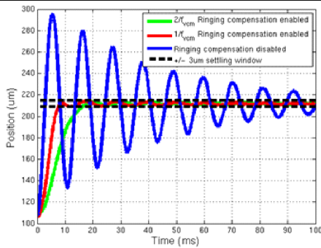
Figure 22. Lens Positions With and Without Ringing Compensation With 100- \mu\text{m} Step on the Lens Position
