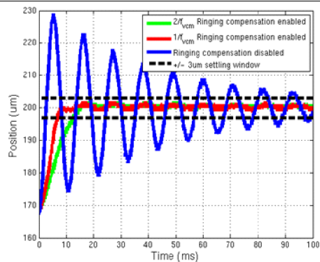
Figure 24. Lens Positions With and Without Ringing Compensation With 30- \mu\text{m} Step on the Lens Position
