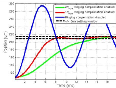
Figure 23. Lens Positions With and Without Ringing Compensation With 100- \mu\text{m} Step on the Lens Position, Zoomed In
