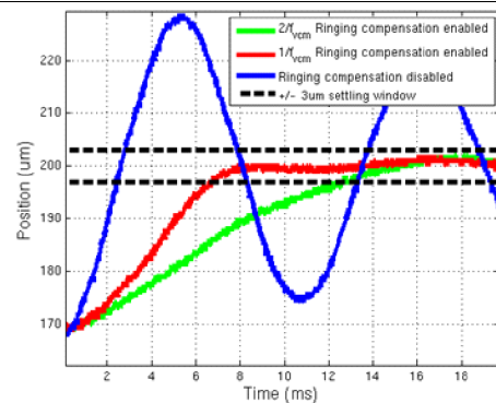
Figure 23. Lens Positions With and Without Ringing Compensation With 100- \mu\text{m} Step on the Lens Position, Zoomed In
