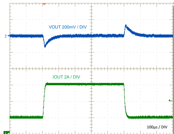
V_{IN} = 48V V_{OUT} = 5V FPWM
