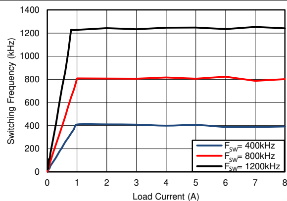
图 6-20. F_{SW} Load Regulation, Mode = DCM, V_{IN} = 12\text{V} , V_{OUT} = 1.2\text{V}
