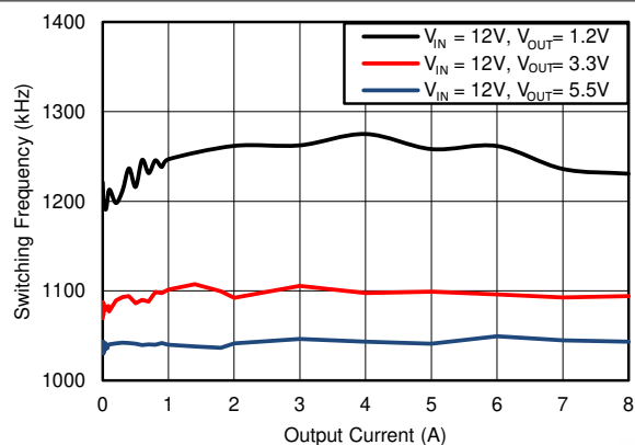
图 6-19. F_{SW} Load Regulation, Mode = FCCM, F_{SW} = 1200\text{kHz}
