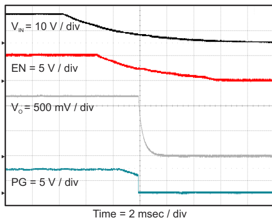
图 8-16. Shut Down Relative to V_{IN} Falling
