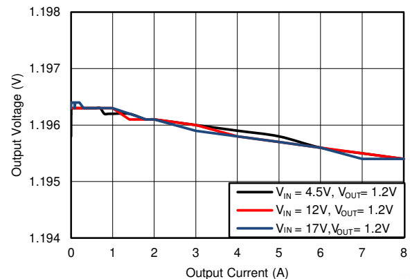
图 6-16. Load Regulation, F_{SW} = 400\text{kHz}
