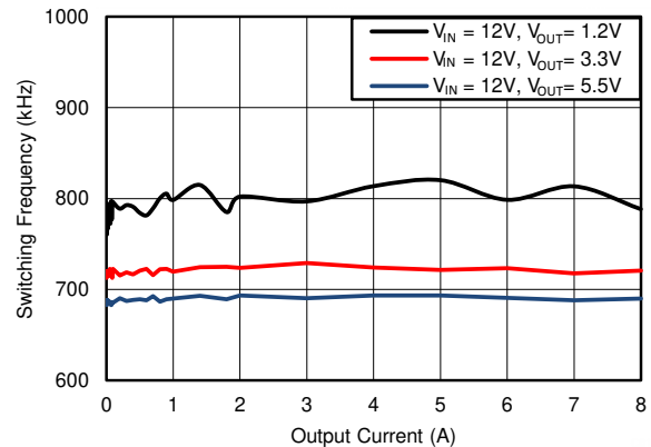
图 6-18. F_{SW} Load Regulation, Mode = FCCM, F_{SW} = 800\text{kHz}
