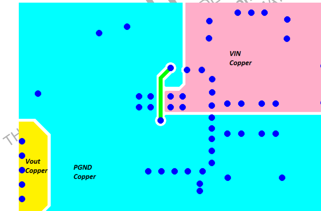
Figure 32. PCB Layout Example (Bottom View)
