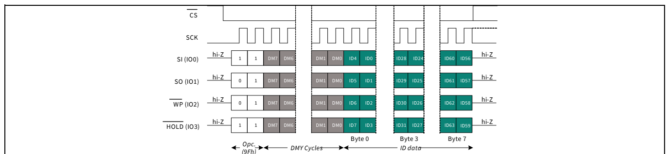
Figure 89 Read device ID (RDID) in QPI mode
