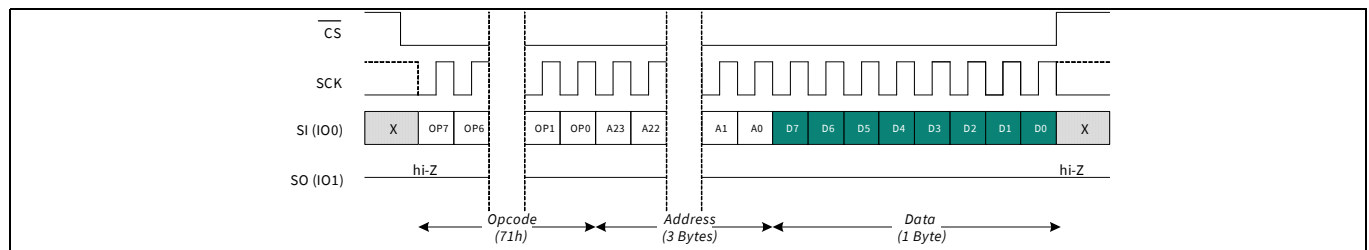
Figure 33 Write Any register (WRAR) in SPI mode
