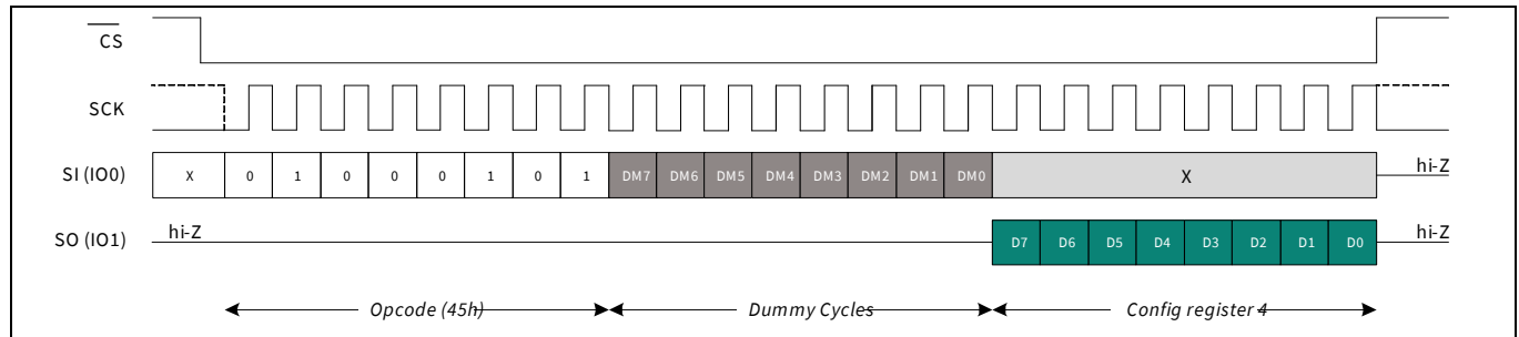
Figure 27 Read CR4 (RDCR4) in SPI mode
