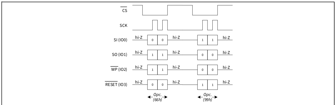
Figure 108 Software reset timing in QPI mode
