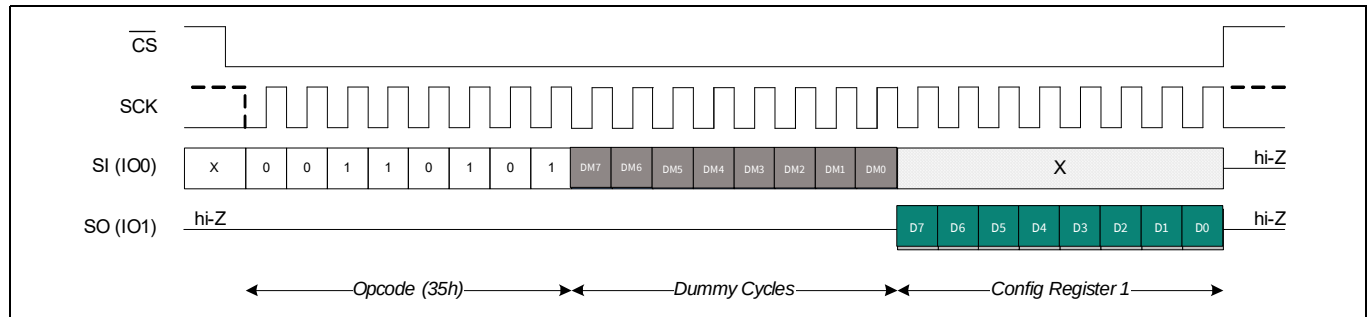
Figure 21 Read CR1 (RDCR1) in SPI mode
