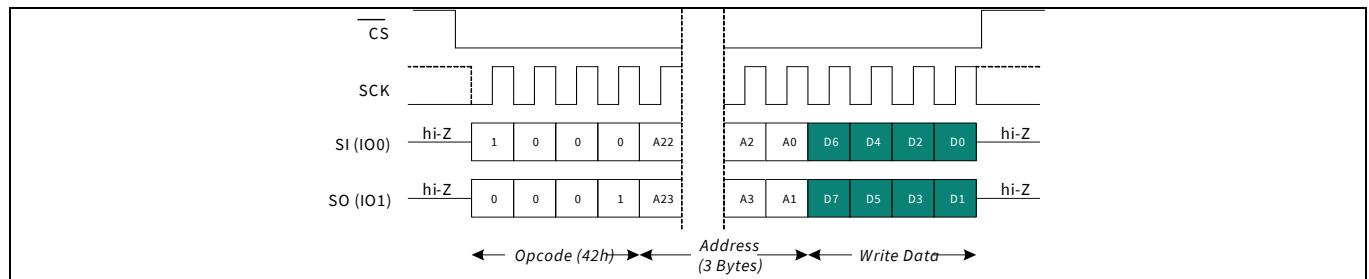
Figure 67 Special sector write (SSWR) in DPI mode (WREN is not shown)
