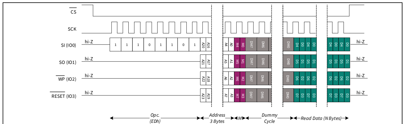
Figure 64 Quad I/O read in DDR (DDRQIOR) – in extended SPI mode
