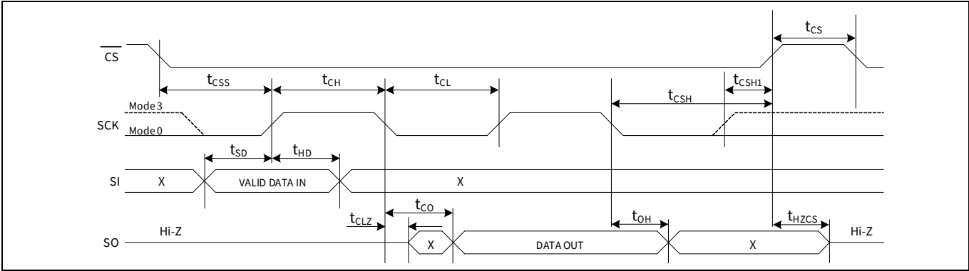
Figure 114 SPI switching timing - single IO, SDR (Mode 0 and Mode 3)
