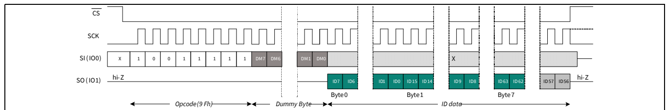
Figure 87 Read device ID (RDID) in SPI mode
