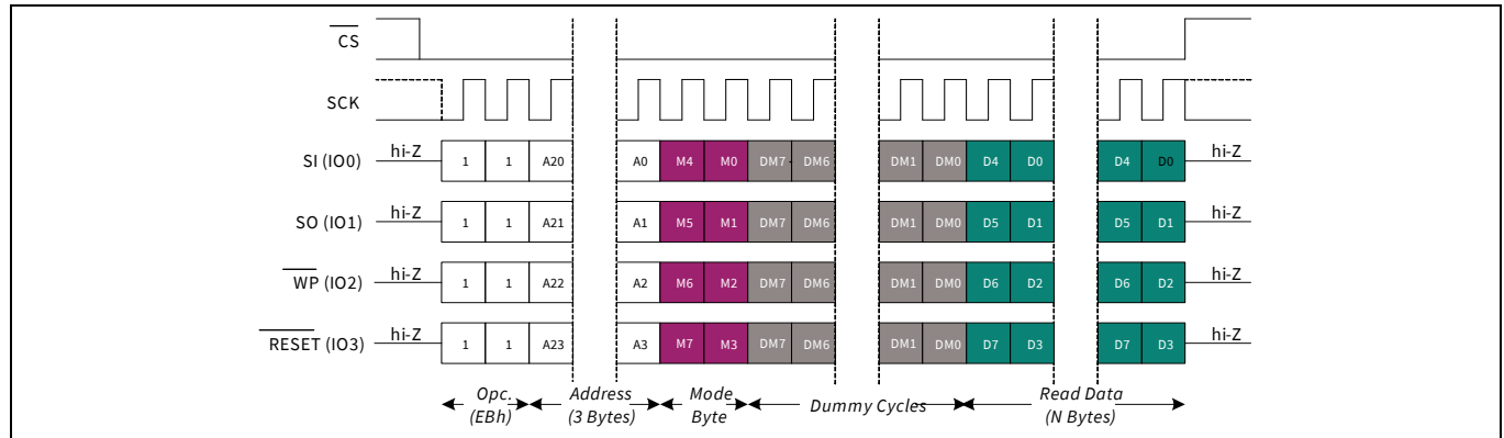
Figure 63 Quad I/O read (QIOR) in QPI mode
