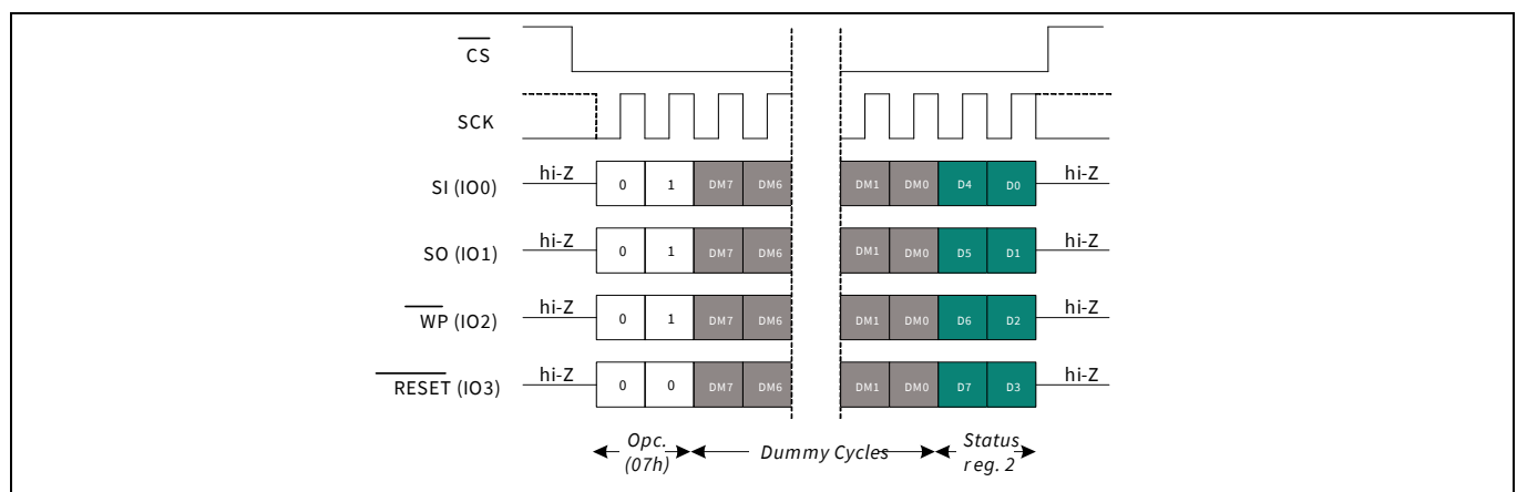
Figure 20 Read SR2 (RDSR2) in QPI mode
