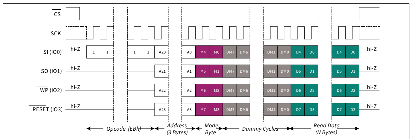
Figure 62 Quad I/O read (QIOR) in extended SPI mode
