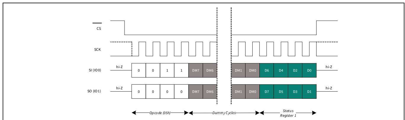
Figure 16 Read SR1 (RDSR1) in DPI mode
