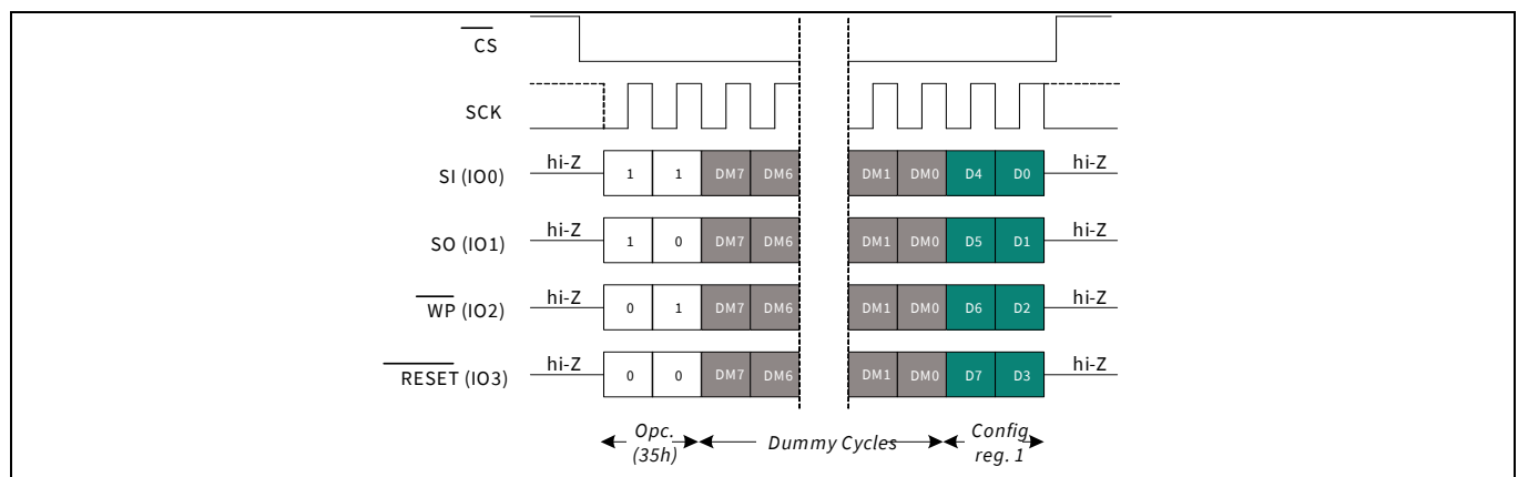
Figure 23 Read CR1 (RDCR1) in QPI mode
