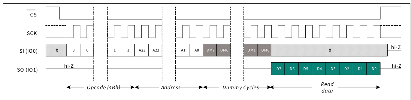
Figure 69 Special sector read (SSRD) in SPI mode
