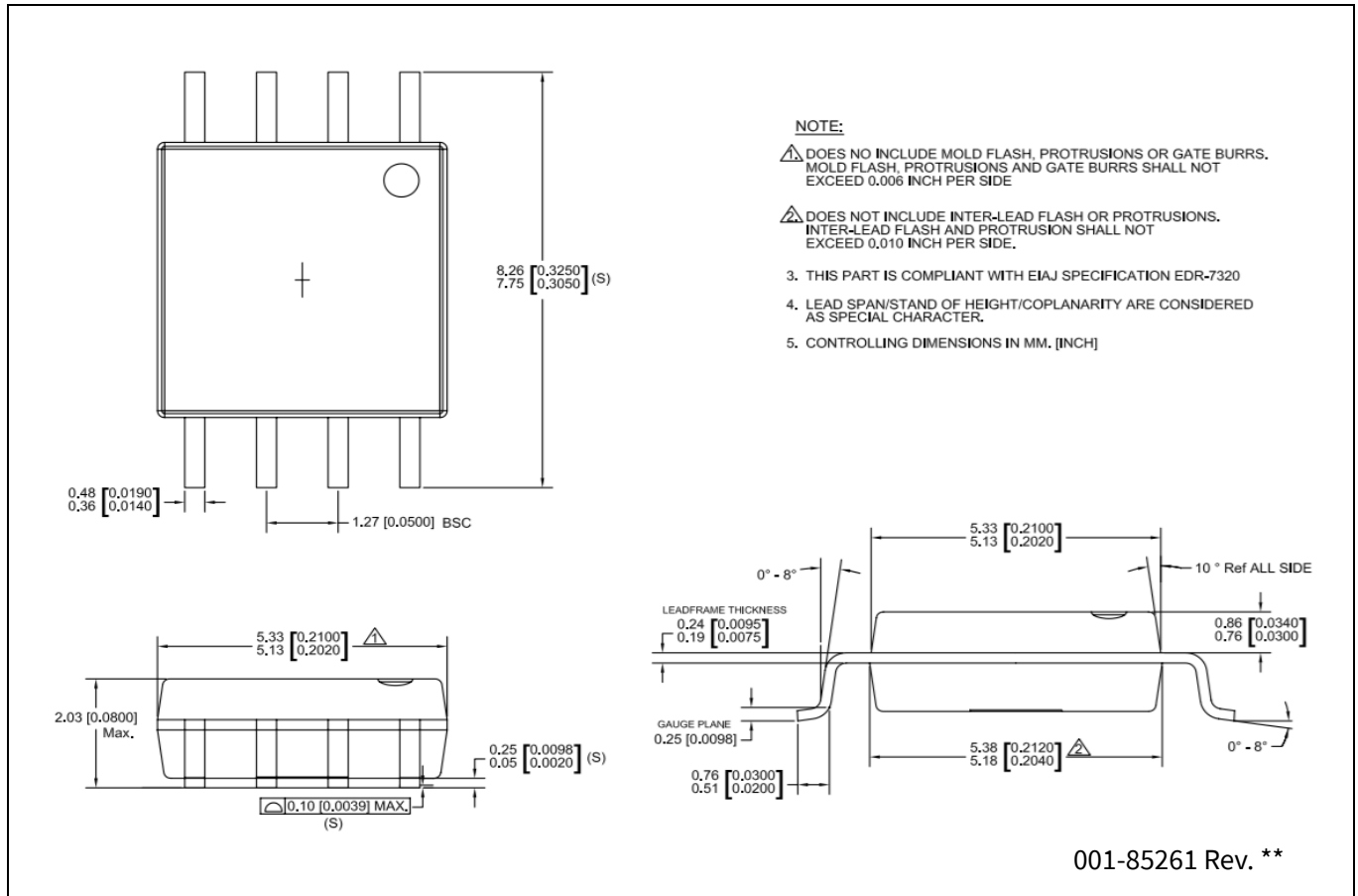
Figure 121 8-pin SOIC (208 MILS) SZ820 package outline (PG-DS0-8)
