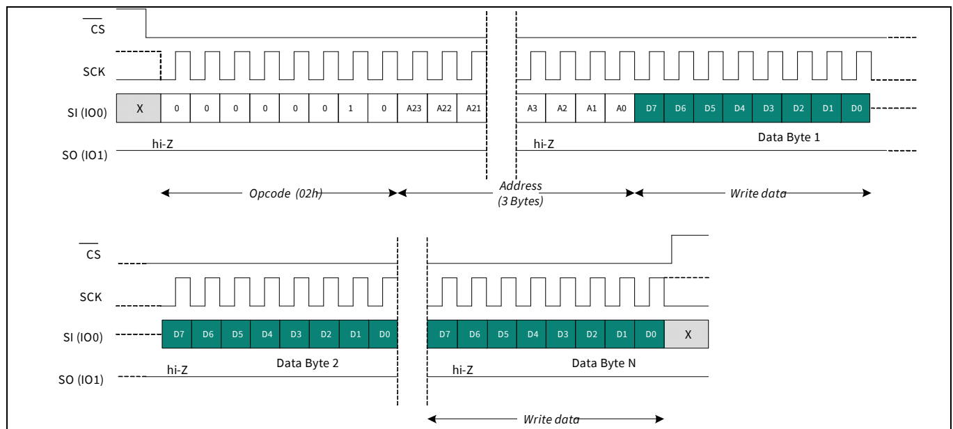
Figure 39 Memory write (WRITE) in SPI mode
