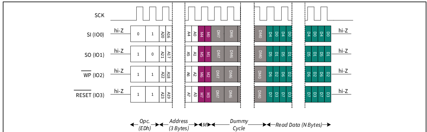
Figure 65 Quad I/O read in DDR (DDRQIOR) – in QPI mode
