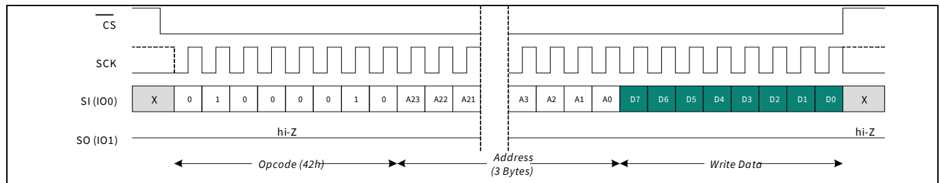
Figure 66 Special sector write (SSWR) in SPI mode (WREN is not shown)
