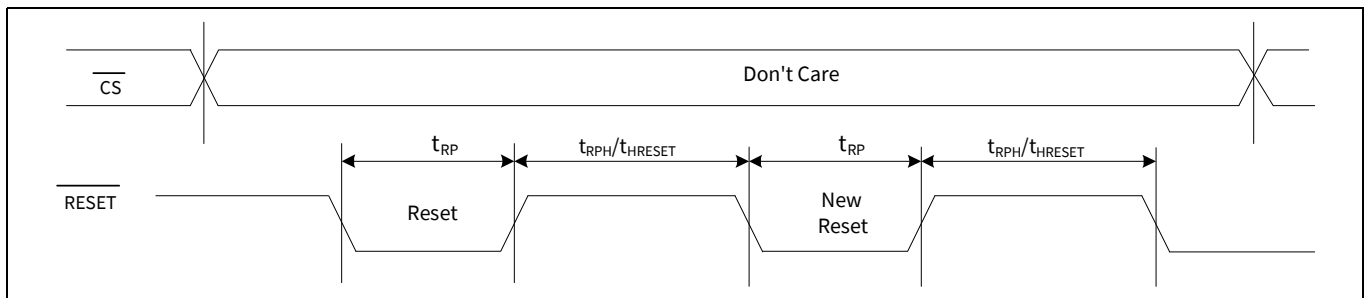
Figure 110 RESET timing - SPI with Quad clear (CR1[1]= '0') and QPI disabled (CR2[6] = '0')
