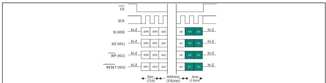
Figure 35 Write any register (WRAR) in QPI mode
