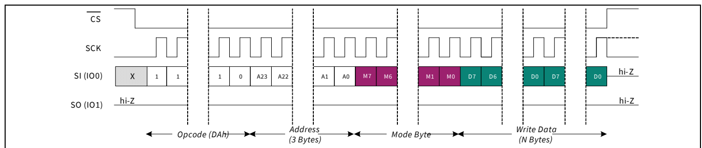
Figure 43 Fast write (FAST_WRITE) in SPI mode
