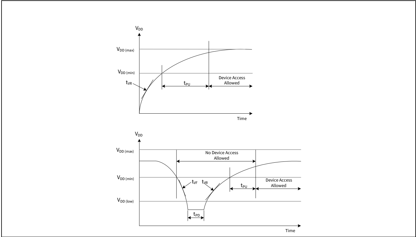
Figure 120 Power cycle timing
