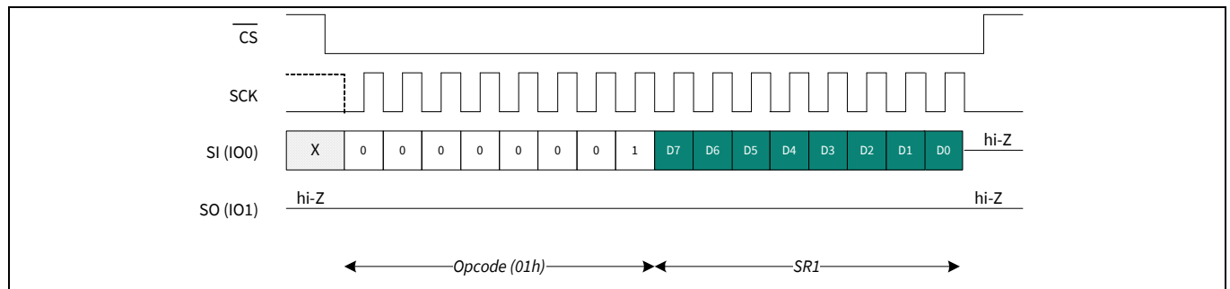
Figure 12 WRSR in SPI mode (WREN not shown)
