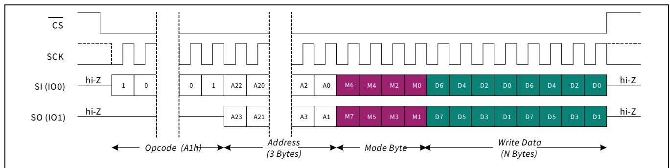
Figure 48 Dual I/O write (DIOW)
