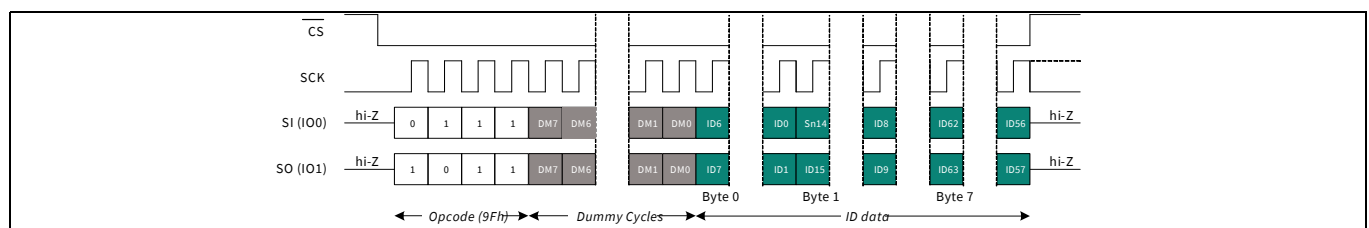
Figure 88 Read device ID (RDID) in DPI mode
