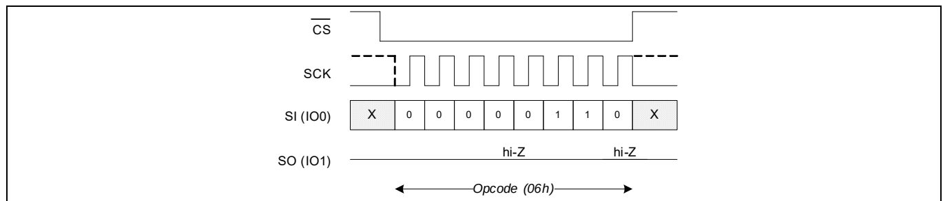
Figure 6 WREN bus configuration in SPI mode
