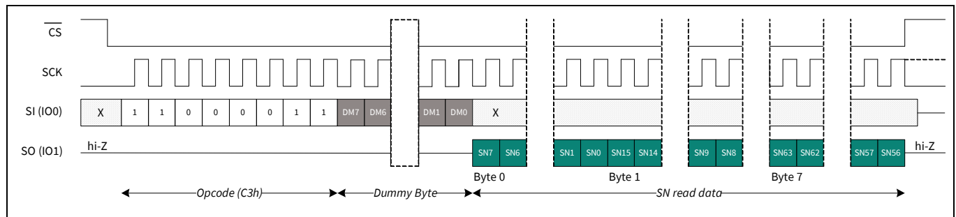
Figure 96 Read serial number (RDSN) in SPI mode
