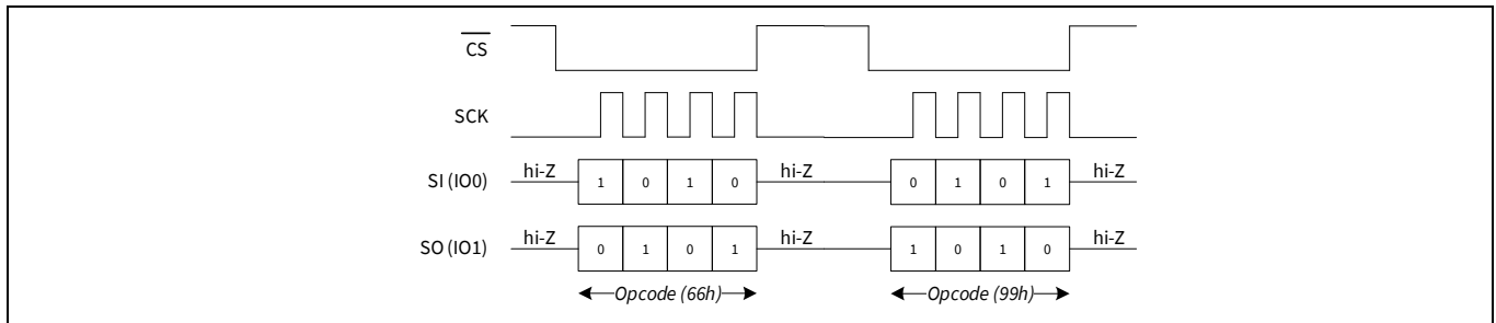
Figure 107 Software reset timing in DPI mode
