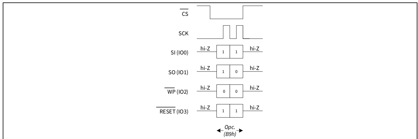
Figure 101 DPD mode operation in QPI mode
