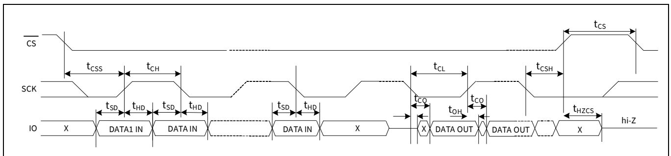
Figure 118 SPI switching timing - multiple I/O, DDR [28]
