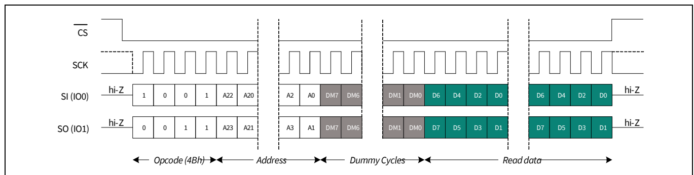
Figure 70 Special sector read (SSRD) in DPI mode
