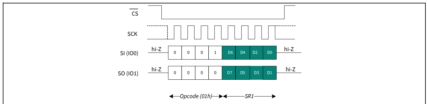
Figure 13 WRSR in DPI mode (WREN not shown)
