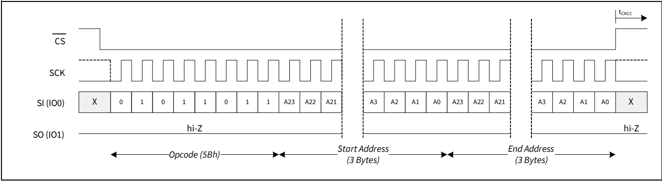
Figure 78 CRC calculation (CRCC) in SPI mode
