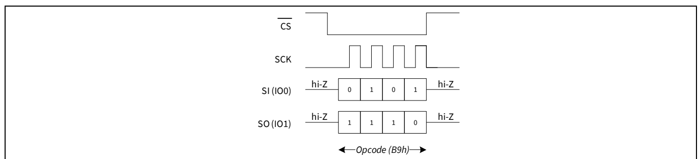
Figure 100 DPD mode operation in DPI mode
