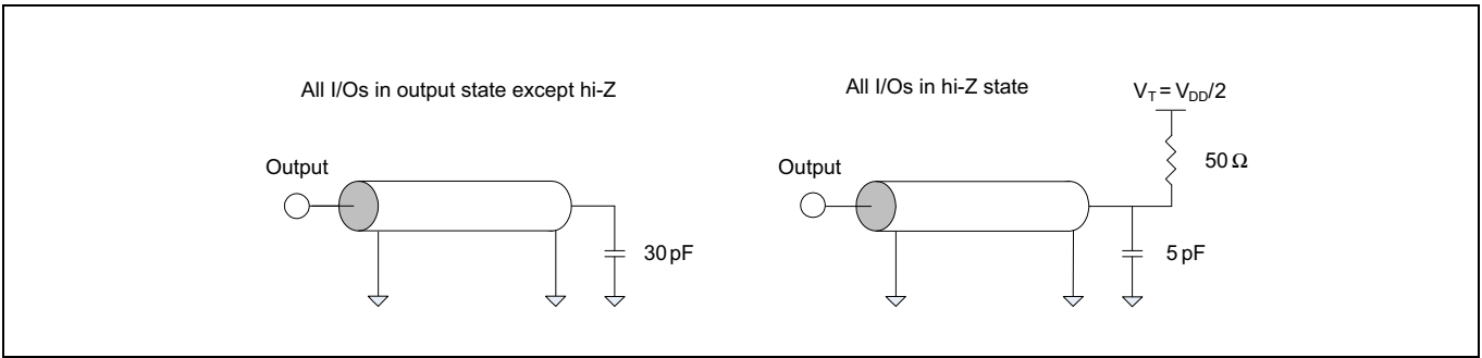
Figure 112 AC test loads
