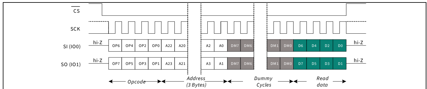
Figure 37 Read Any register (RDAR) in DPI mode
