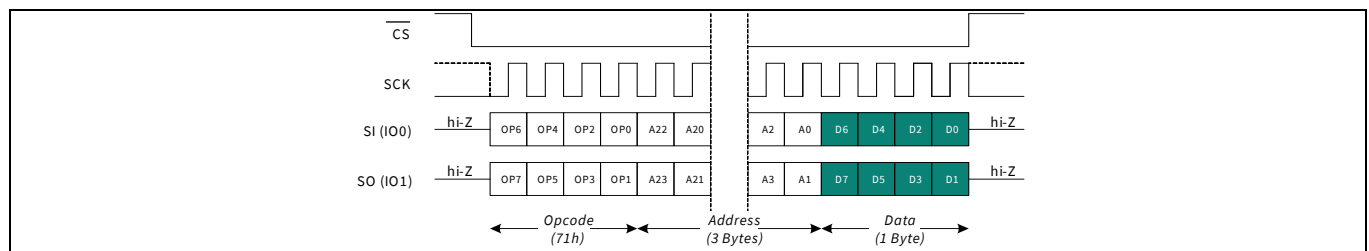
Figure 34 Write Any register (WRAR) in DPI mode
