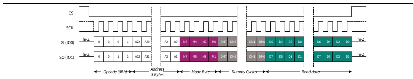
Figure 56 FAST_READ in DPI mode
