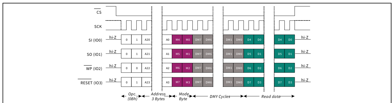
Figure 57 FAST_READ in QPI mode
