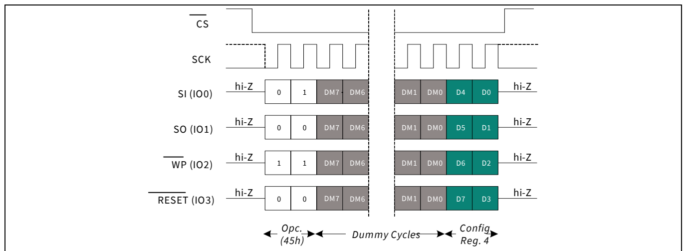
Figure 29 Read CR4 (RDCR4) in QPI mode
