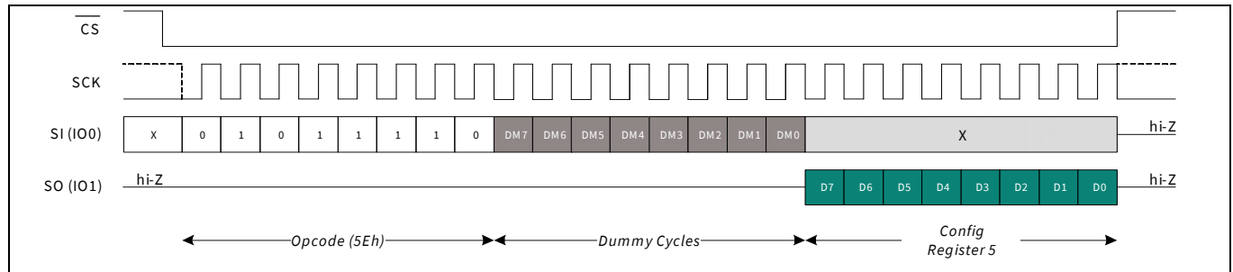
Figure 30 Read CR5 (RDCR5) in SPI mode
