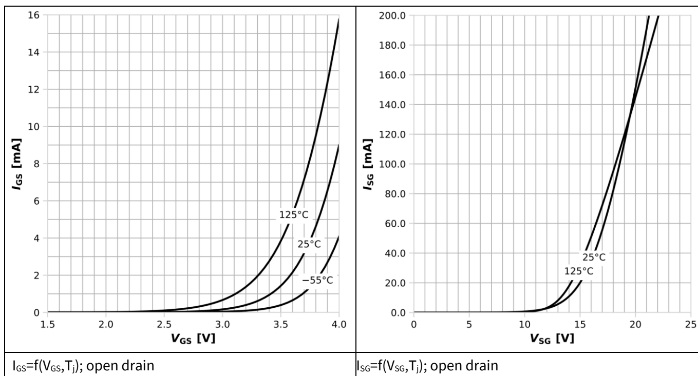
Figure 12 Typical gate characteristics forward and reverse
