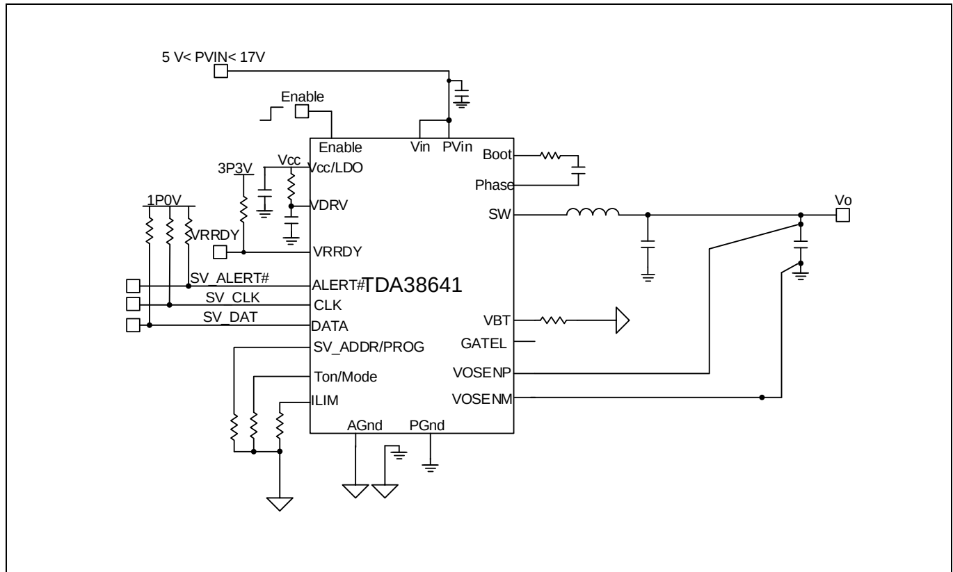
Figure 4 TDA38641 Application Circuit in VOUT_SCALE_LOOP 1:1 & SVID mode ( 0\text{ V} \leq \text{VID} \leq 2.56\text{ V} )
