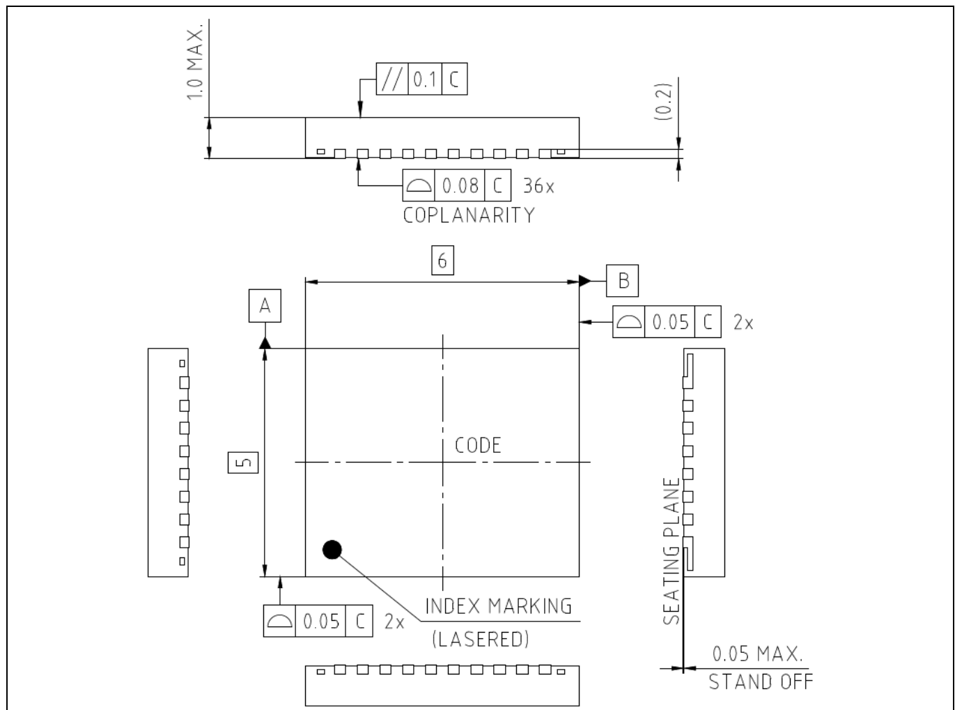
Figure 25 Package view
