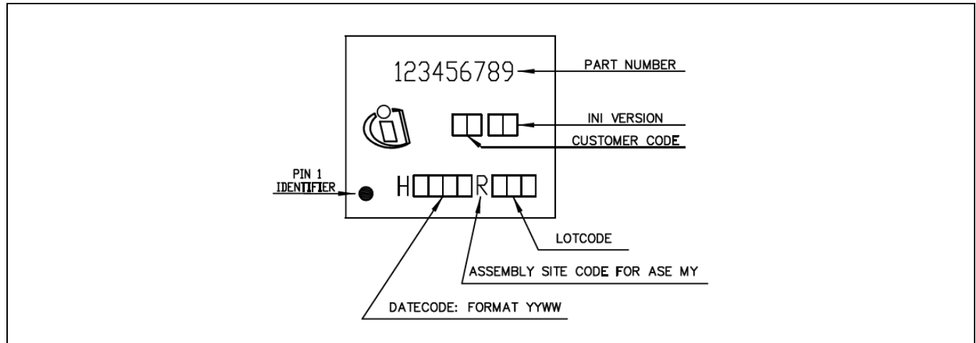
Figure 24 Package Marking
