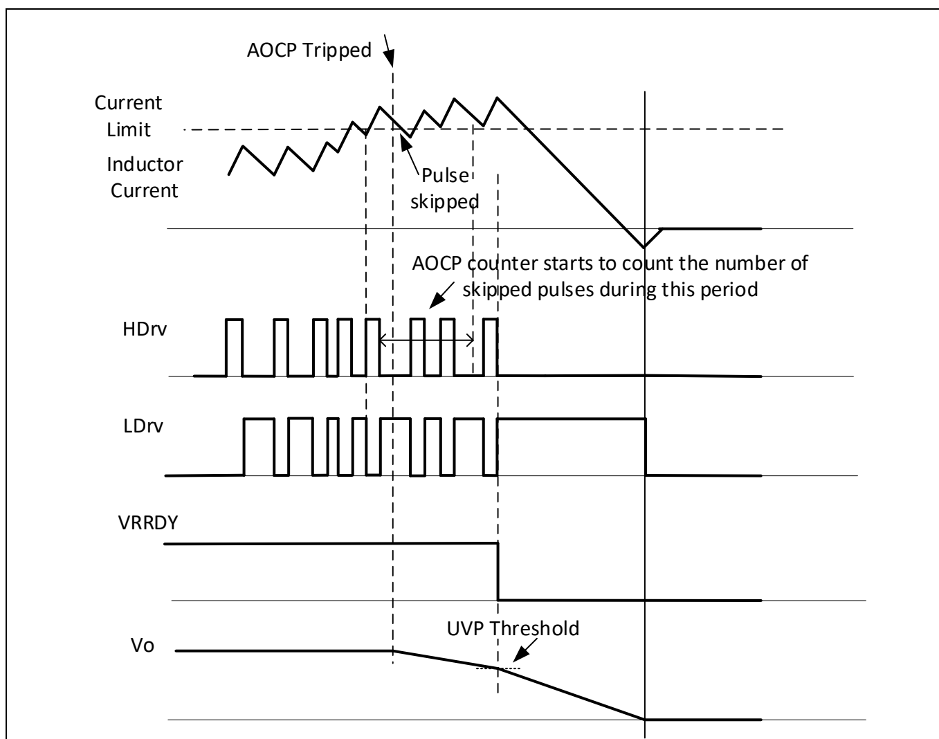
Figure 17 AOCP response timing diagram.
