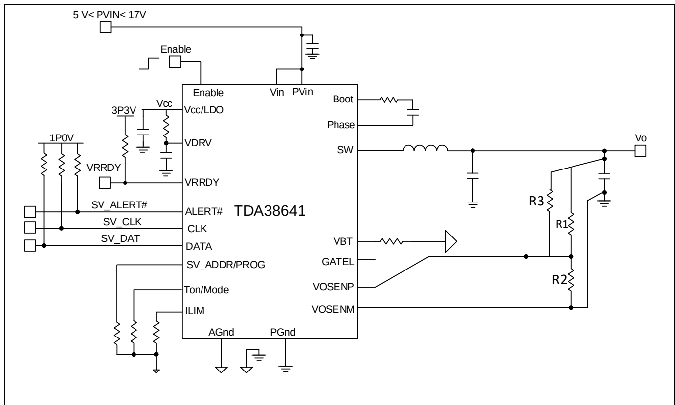
Figure 5 TDA38641 Application Circuit in VOUT_SCALE_LOOP 1:2 & SVID mode ( 2.56\text{ V} \leq \text{VID} \leq 3.04\text{ V} )
