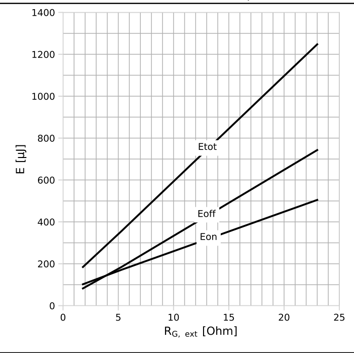
Diagram 19: Typ. Switching Losses vs R_{G,ext}
