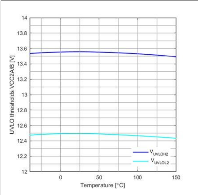
Figure 10 V_{UVLOH2} and V_{UVL0L2} (2EDR3146XQE) vs. temperature
