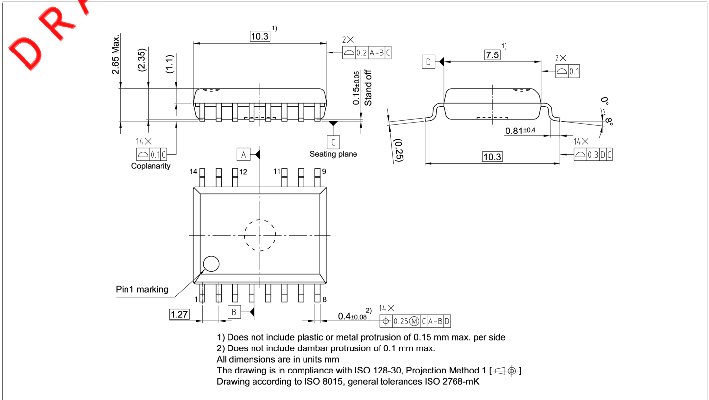
Figure 43 PG-DSO-14-79 (300 mil) outline
