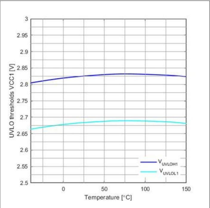
Figure 9 V_{UVLOH1} and V_{UVL0L1} vs. temperature
