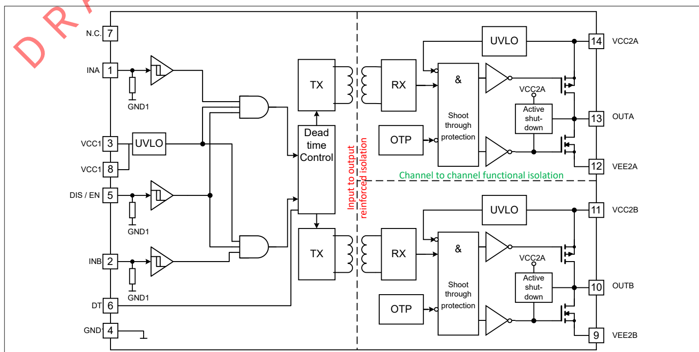
Figure 2 Block diagram
