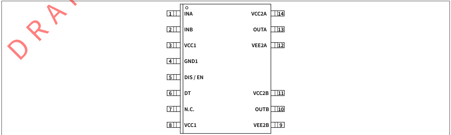
Figure 3 LDSO-14-2 (top view)
