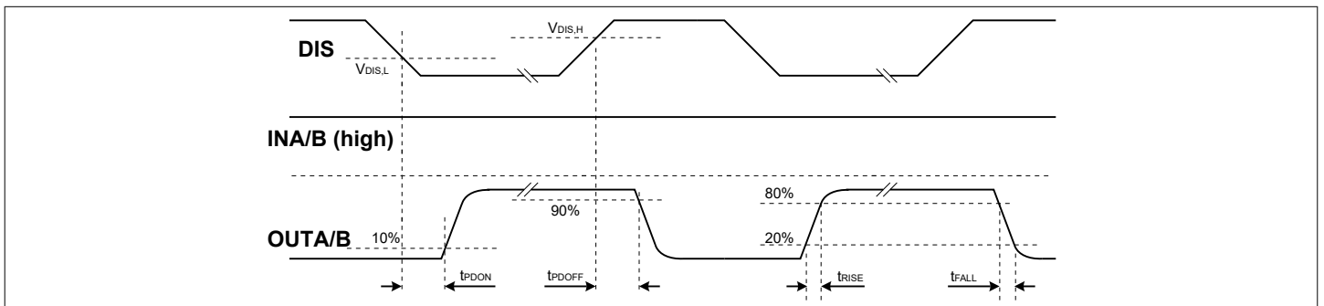
Figure 29 Propagation delay for the DIS pin
