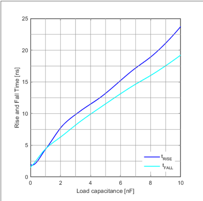
Figure 20 t_{RISE} & t_{fall} vs. C_{LOAD}
