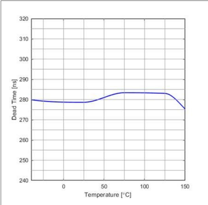
Figure 22 t_{DT} vs. temperature @ R_{DT} = 30\text{k}\Omega
