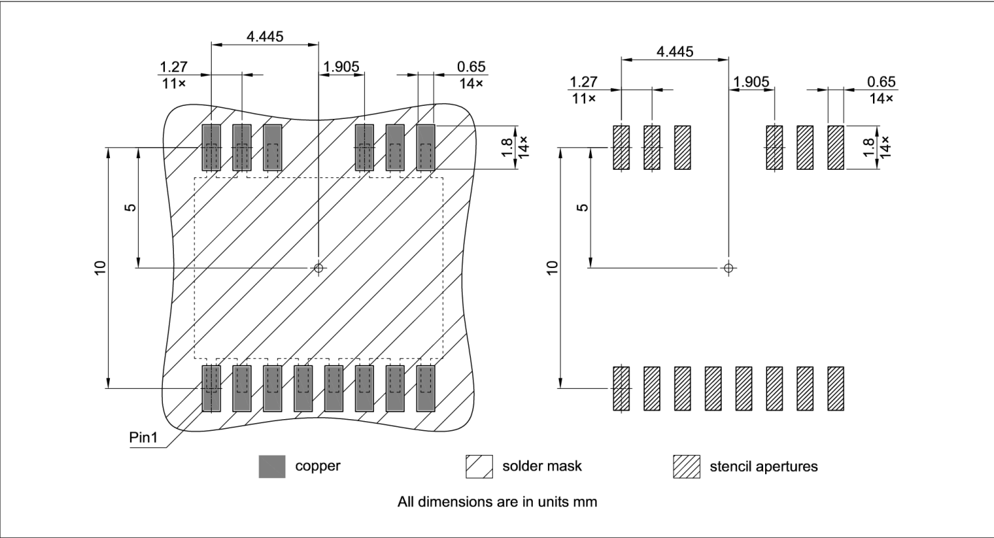
Figure 44 PG-DSO-14-79 (300 mil) recommended footprint
