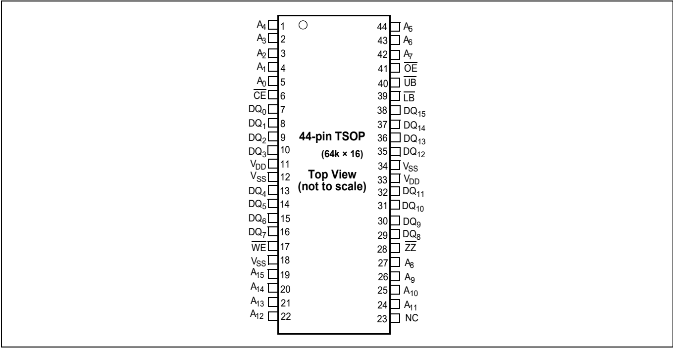
Figure 1 44-pin TSOP (64k × 16) pinout (top view)
