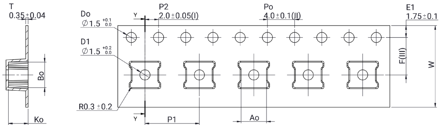
SECTION Y-Y
