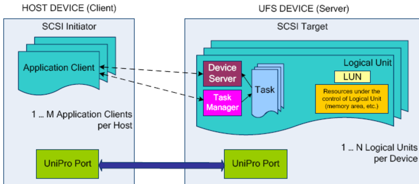
Figure 2-3 UFS SCSI Domain
