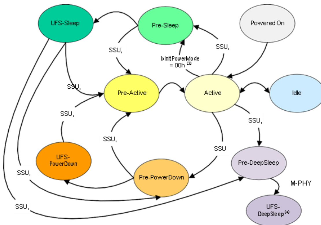
Figure 2-2 Power Mode state Machine
