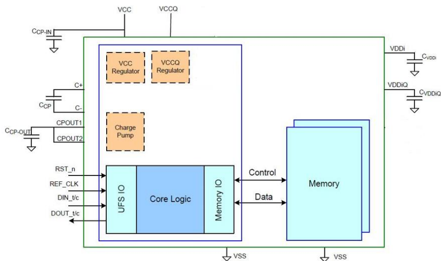
Figure 1-1 UFS Block Diagram
