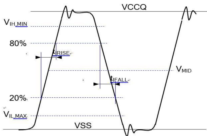
Figure 2-1 Clock input levels, rise time and fall time
