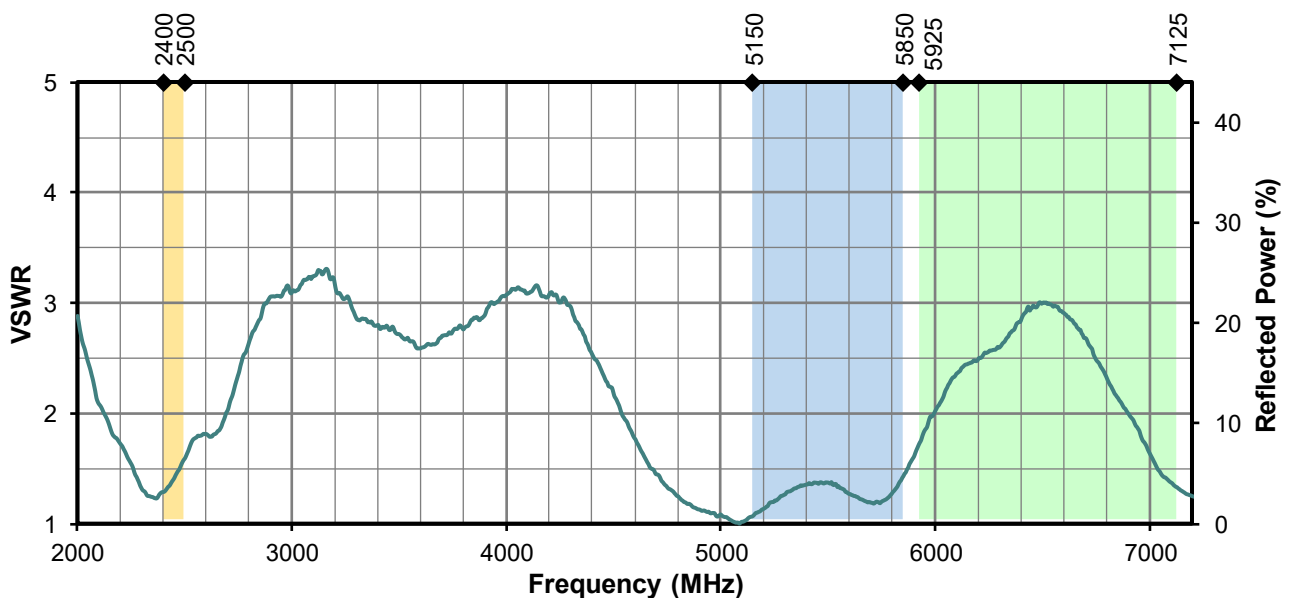
Figure 5. Antenna VSWR, Straight without ground plane
