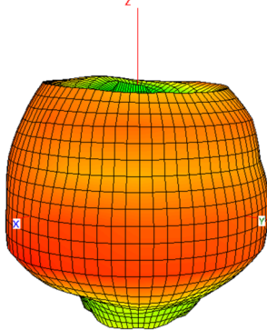
5550 MHz
