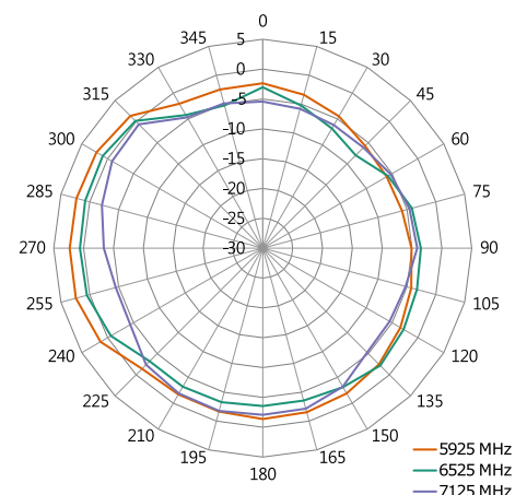
XY-Plane Gain
