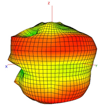
5850 MHz
