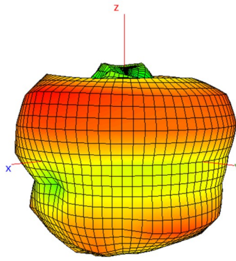
5550 MHz
