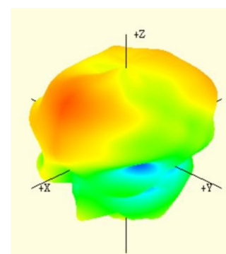
1189 MHz
