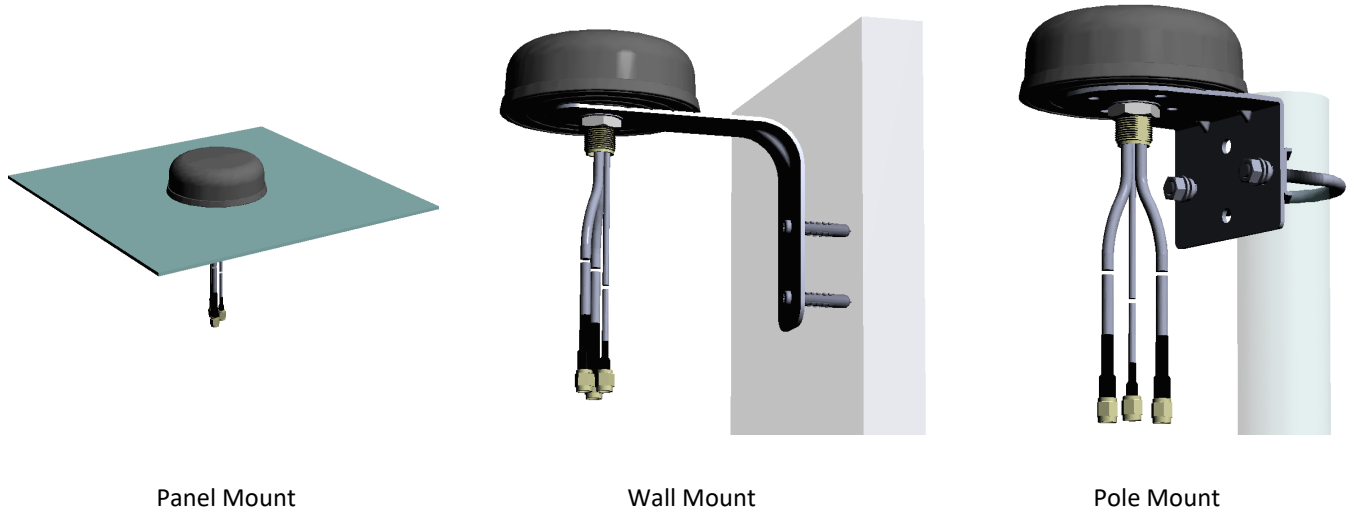
Figure 3. Antenna Installation
