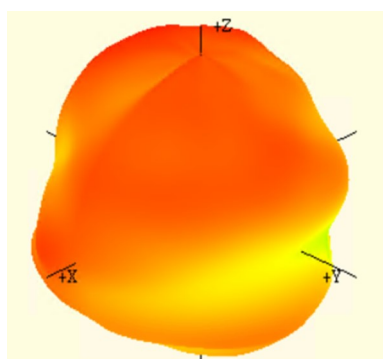
1176.45 MHz
