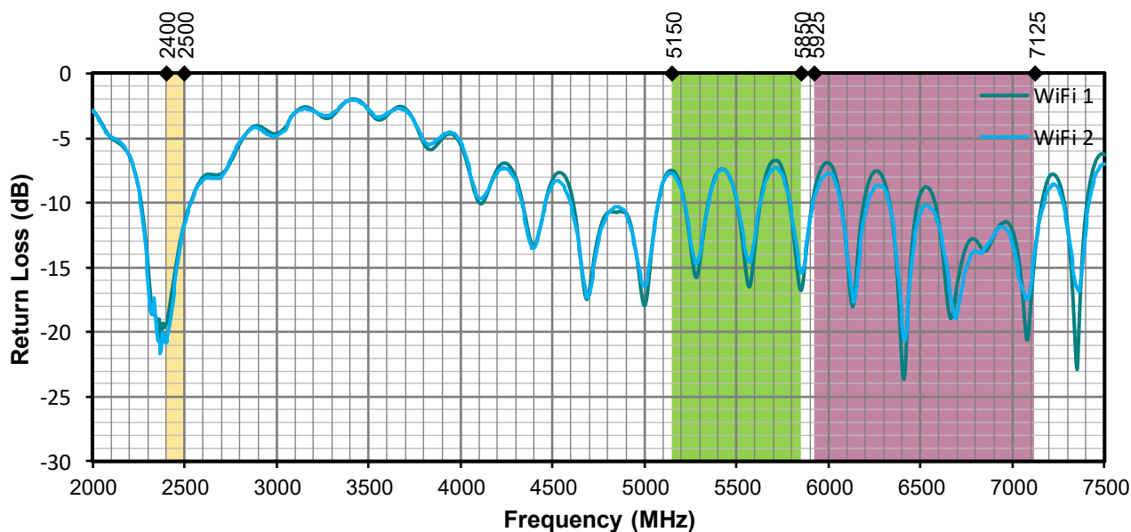
Figure 21. Antenna Return Loss with Ground Plane, WiFi
