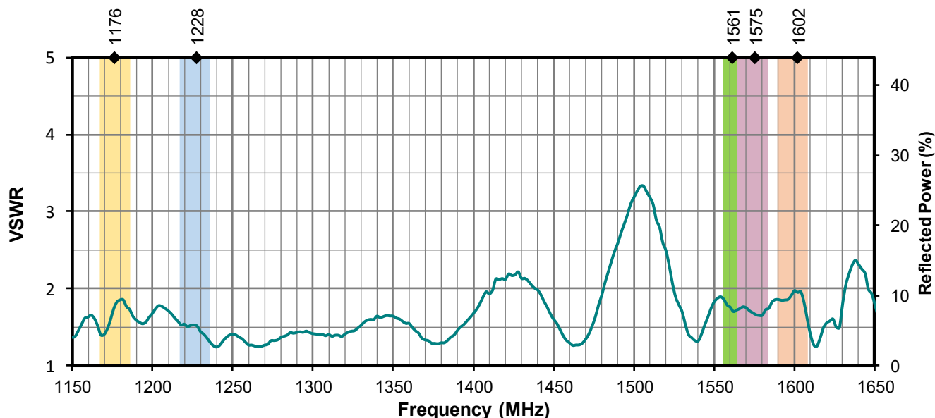
Figure 27. Antenna VSWR with Ground Plane, GNSS
