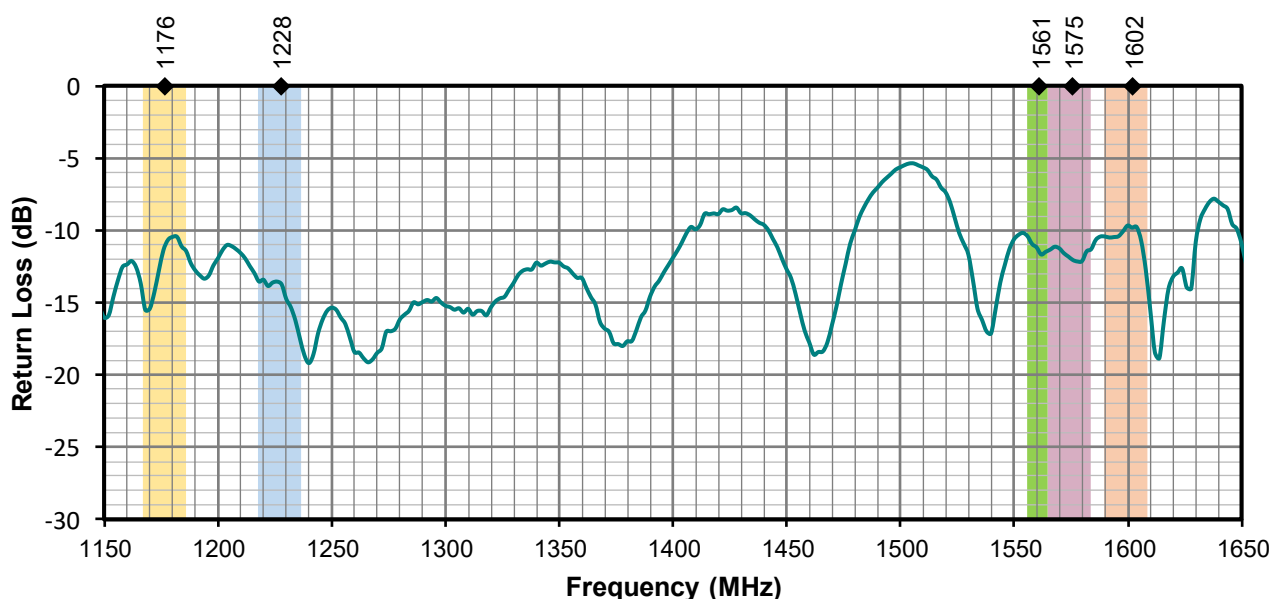
Figure 28. Antenna Return Loss with Ground Plane, GNSS
