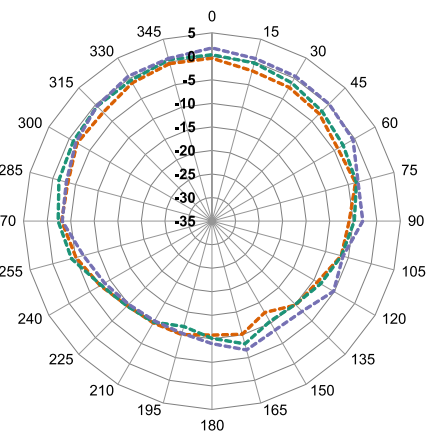
1575.42 MHz
