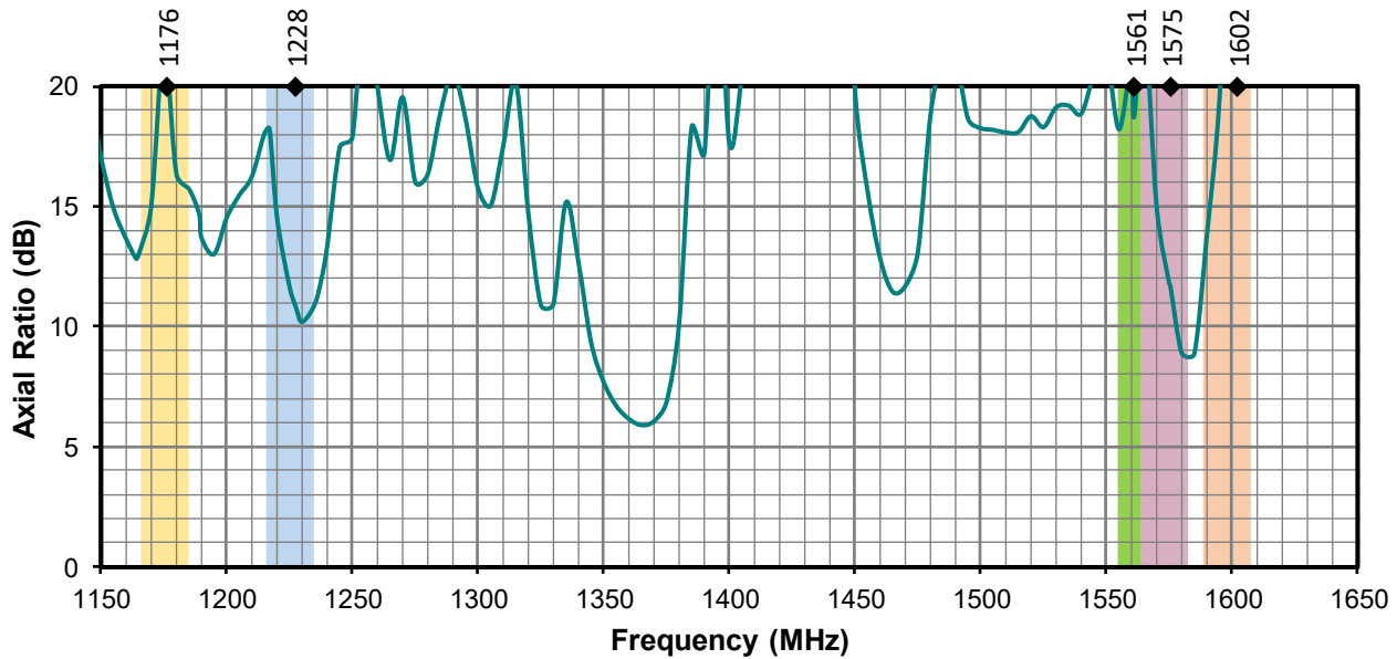
Figure 31. Antenna Axial Ratio with Ground Plane, GNSS
