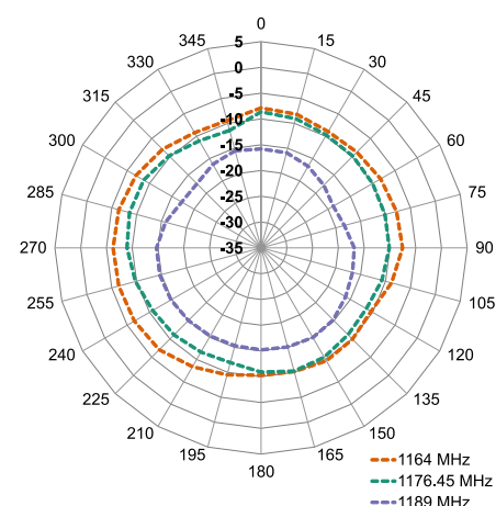
XY-Plane Gain
