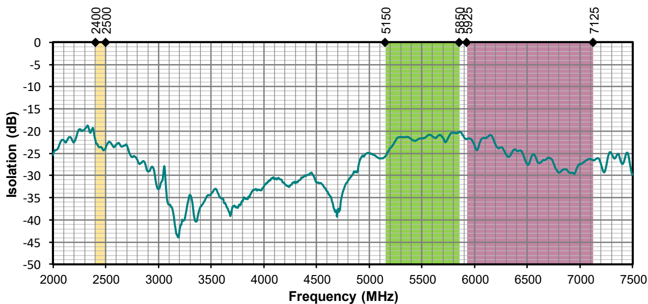
Figure 25. Antenna Isolation with Ground Plane, WiFi
