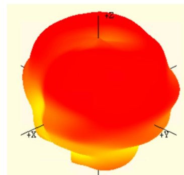
1602 MHz
