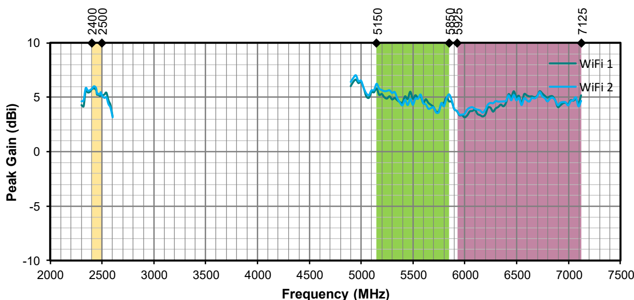
Figure 22. Antenna Peak Gain with Ground Plane, WiFi
