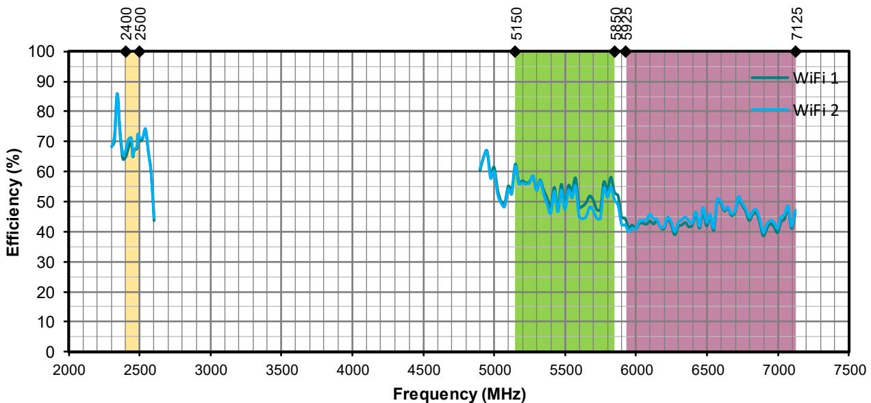
Figure 24. Antenna Efficiency with Ground Plane, WiFi
