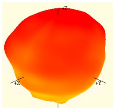
1575.42 MHz
