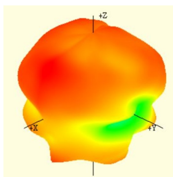
1176.45 MHz
