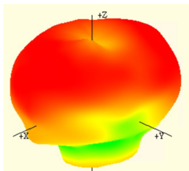
1575.42 MHz
