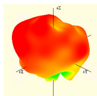
2500 MHz
