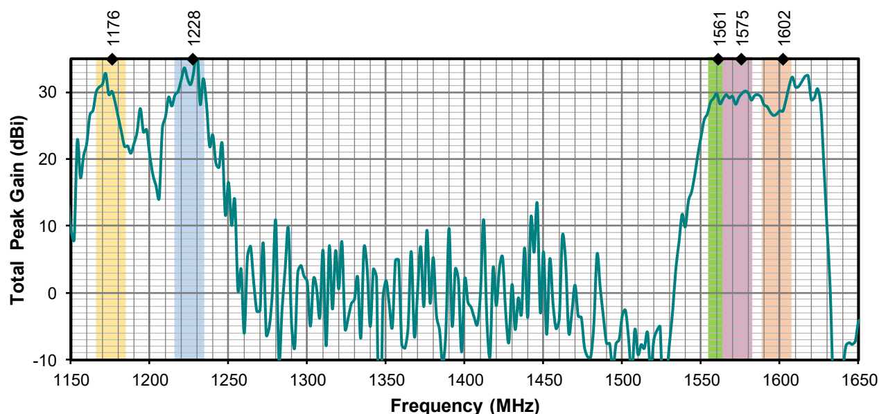
Figure 29. Antenna Total Peak Gain with Ground Plane, GNSS
