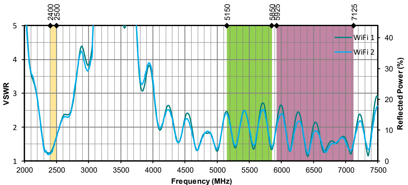
Figure 20. Antenna VSWR with Ground Plane, WiFi
