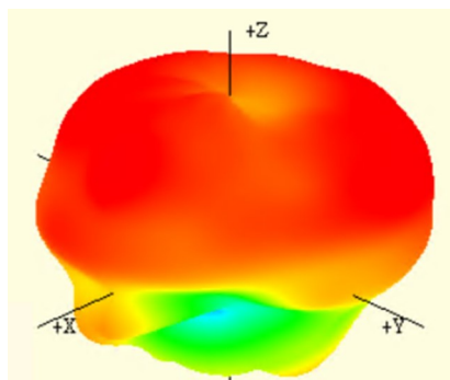
1561 MHz
