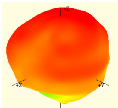
1561 MHz
