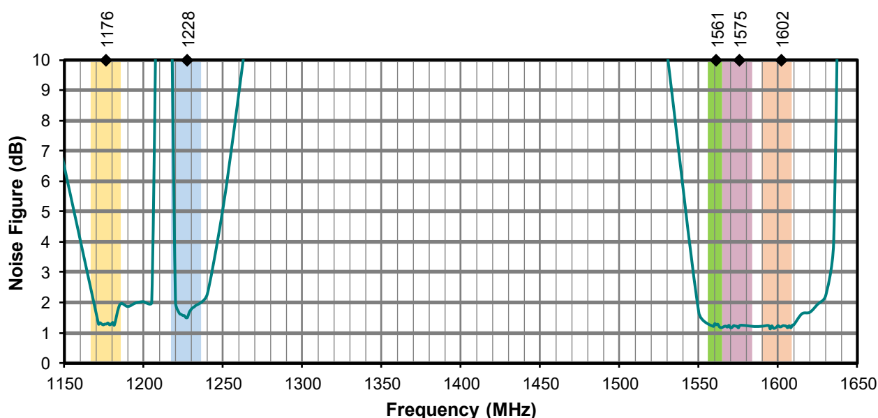
Figure 30. Antenna Noise Figure with Ground Plane, GNSS
