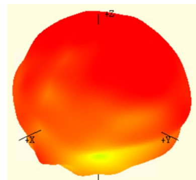
1602 MHz
