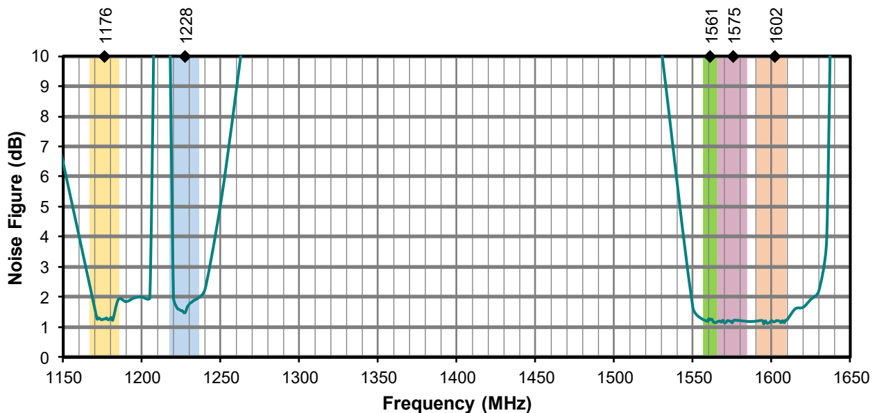
Figure 16. Antenna Noise Figure, GNSS
