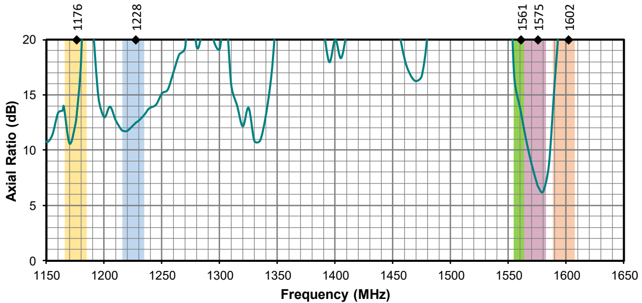
Figure 17. Antenna Axial Ratio, GNSS
