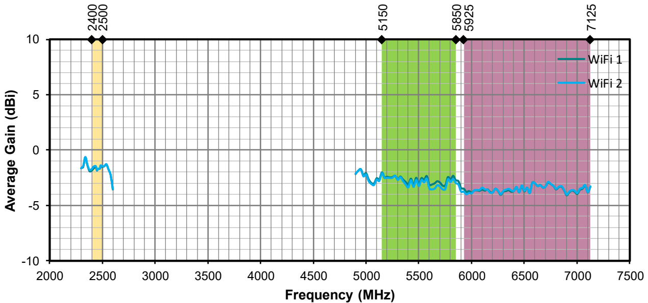
Figure 23. Antenna Average Gain with Ground Plane, WiFi
