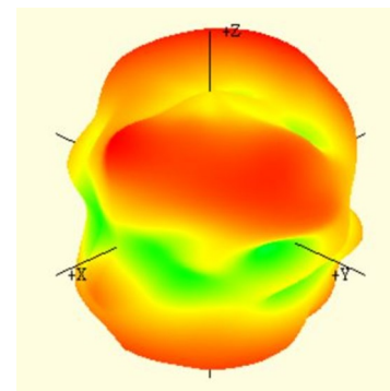
1238 MHz
