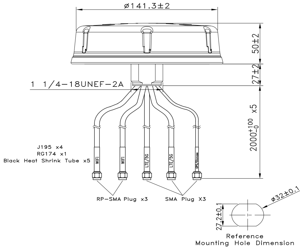
Figure 2. Antenna Dimensions
