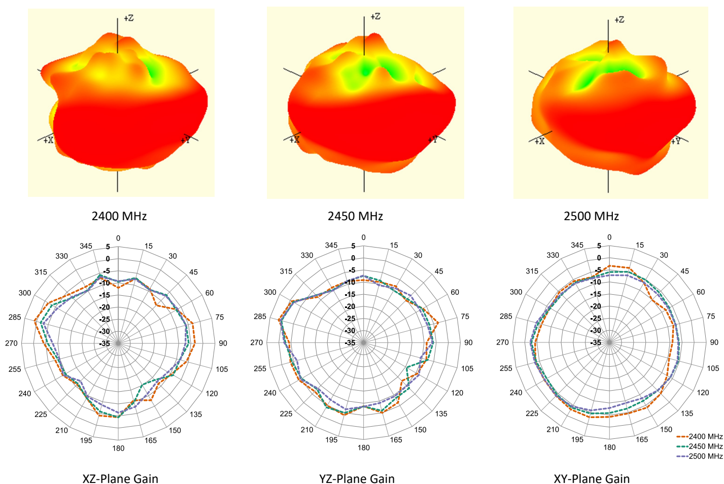
Figure 18-2. Antenna Radiation Patterns, WiFi
