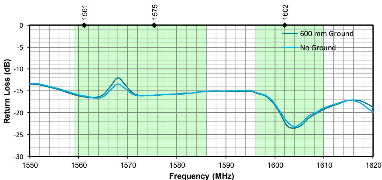
Figure 20. Antenna Return Loss, GNSS
