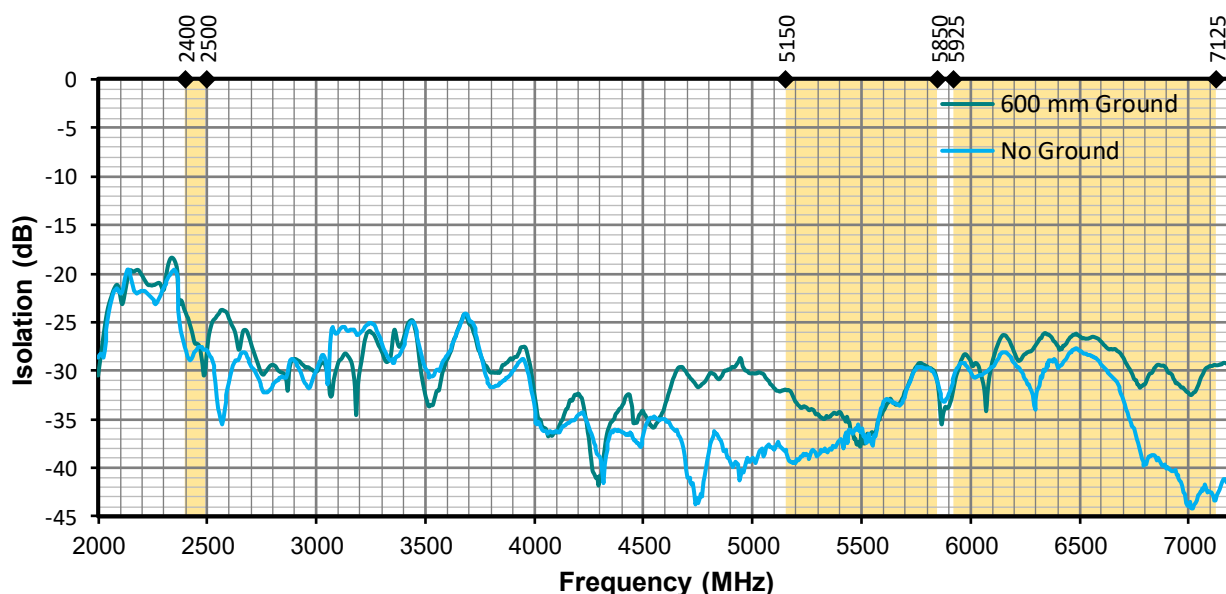
Figure 17. Antenna Isolation, WiFi
