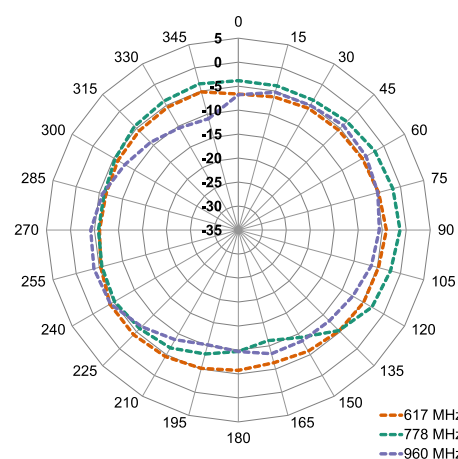
XY-Plane Gain
