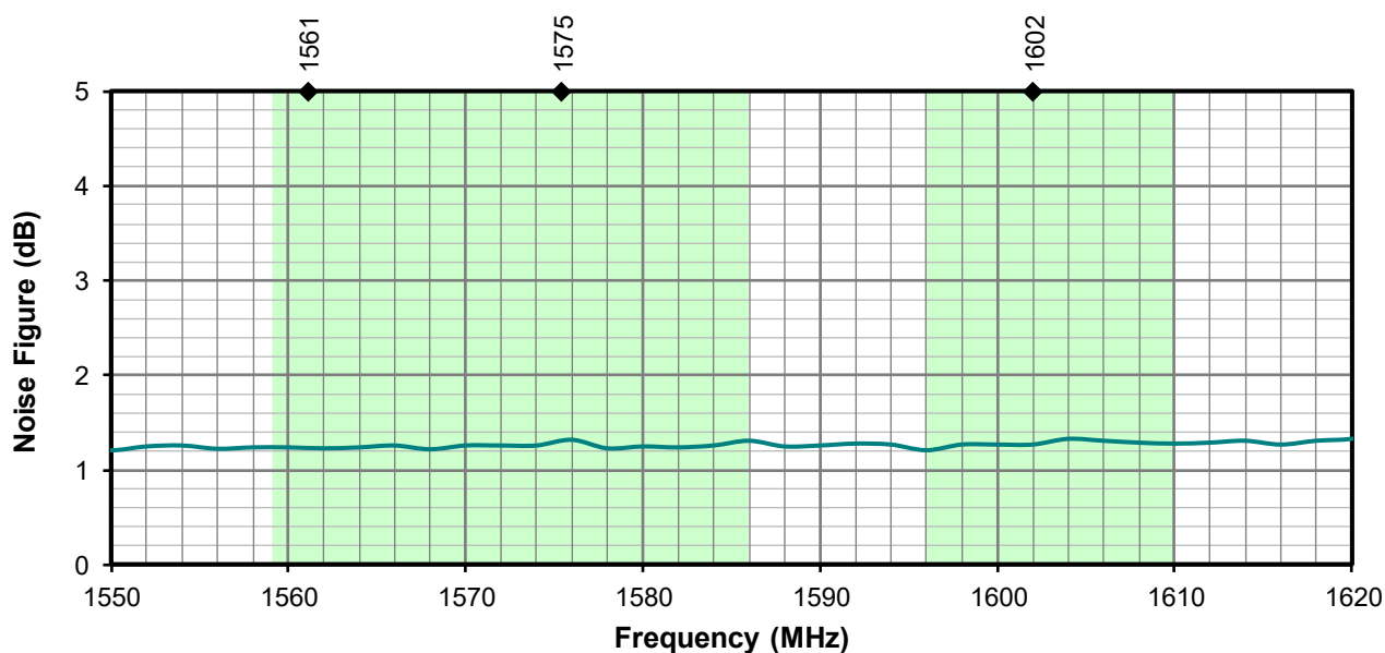
Figure 22. Noise Figure, GNSS
