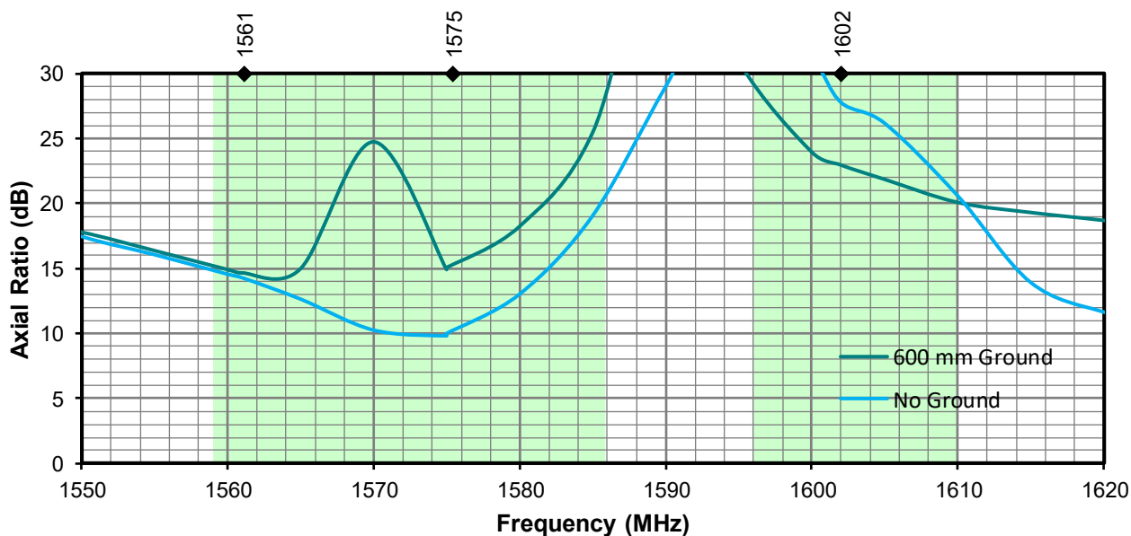
Figure 23. Antenna Axial Ratio, GNSS
