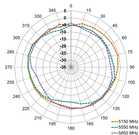
XY-Plane Gain
