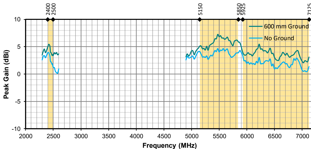
Figure 14. Antenna Peak Gain, WiFi
