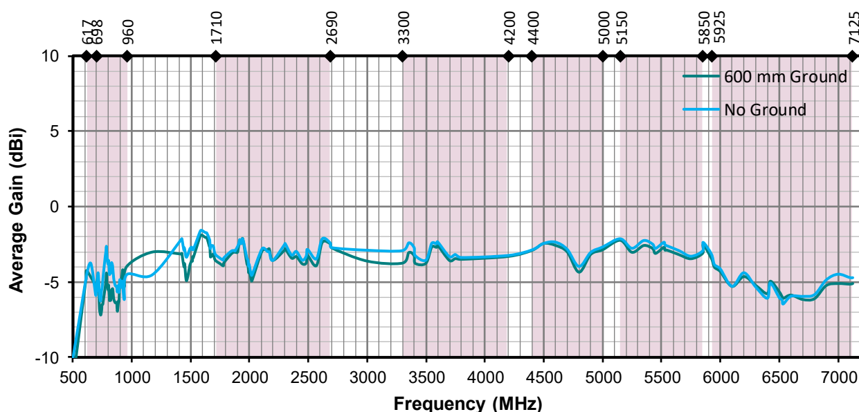
Figure 8. Antenna Average Gain, 5G/LTE
