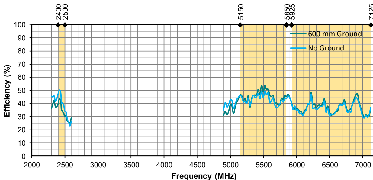
Figure 16. Antenna Efficiency, WiFi
