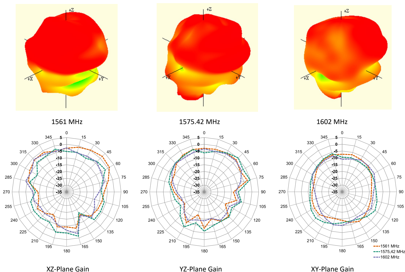
Figure 24-2. Passive Antenna Radiation Patterns, GNSS
