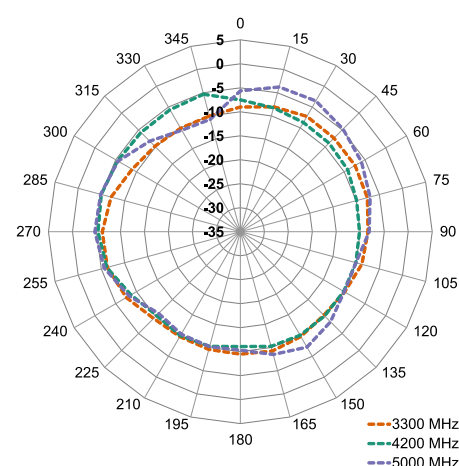
XY-Plane Gain
