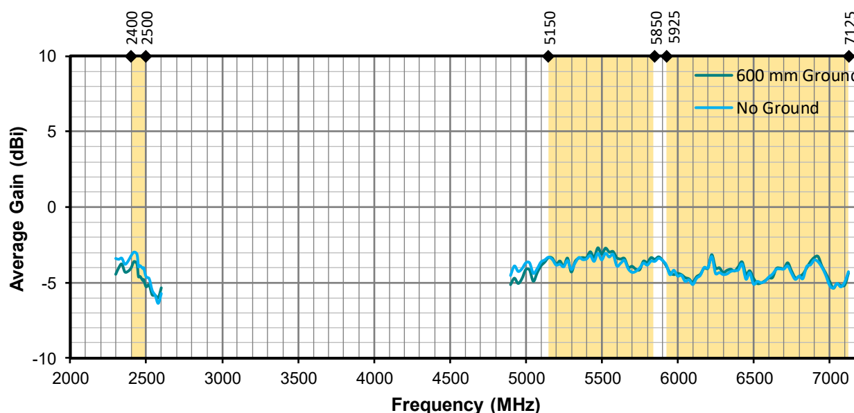
Figure 15. Antenna Average Gain, WiFi
