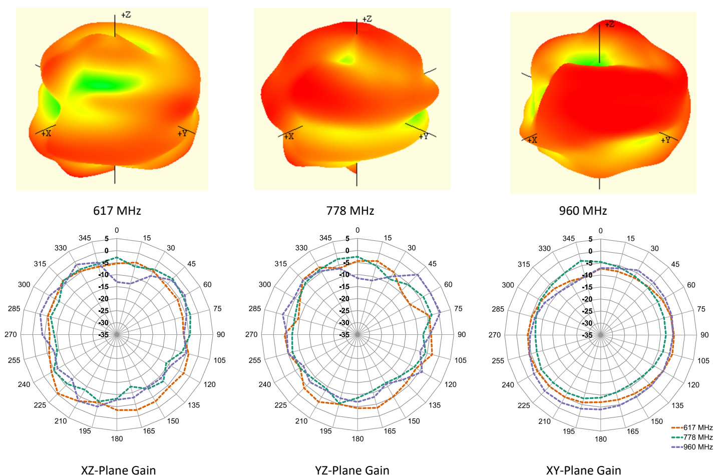
Figure 11-2. Antenna Radiation Patterns, 5G/LTE
