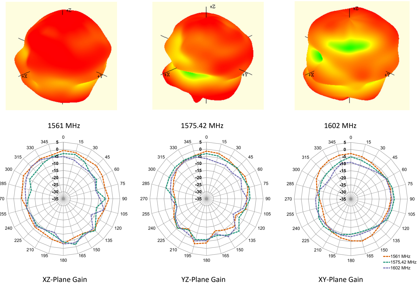
Figure 24. Passive Antenna Radiation Patterns, GNSS
