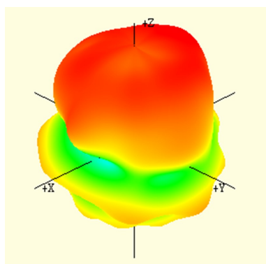
1575.42 MHz
