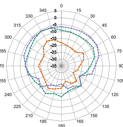
1176.45 MHz
