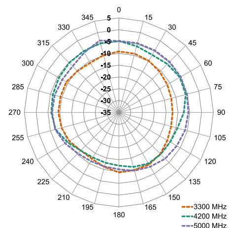
XY-Plane Gain
