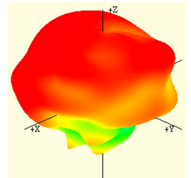
5000 MHz
