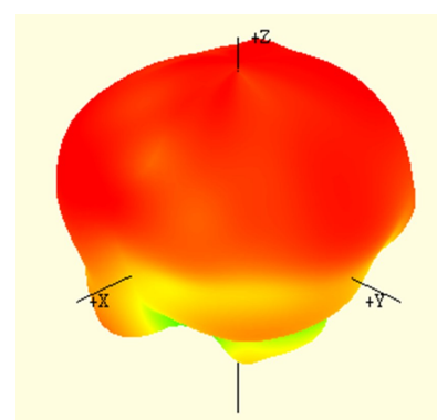
1189 MHz
