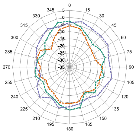
1561 MHz
