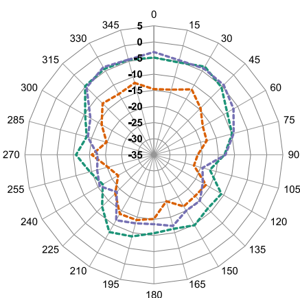
1575.42 MHz
