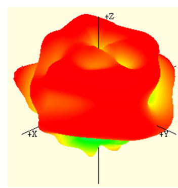
5850 MHz
