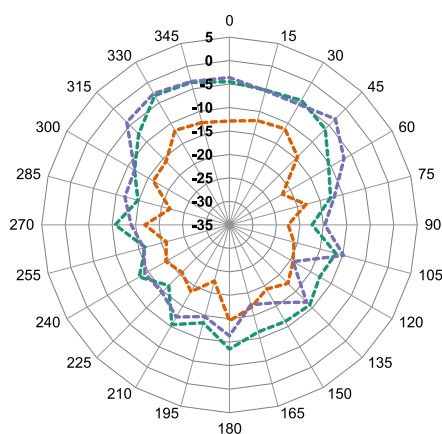
1561 MHz
