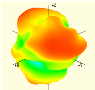
1561 MHz
