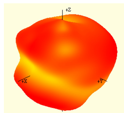
960 MHz
