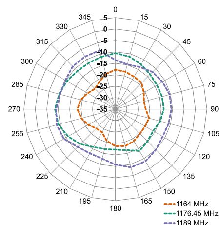
XY-Plane Gain
