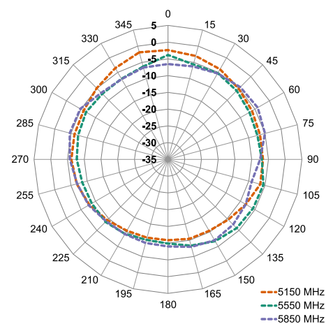
XY-Plane Gain
