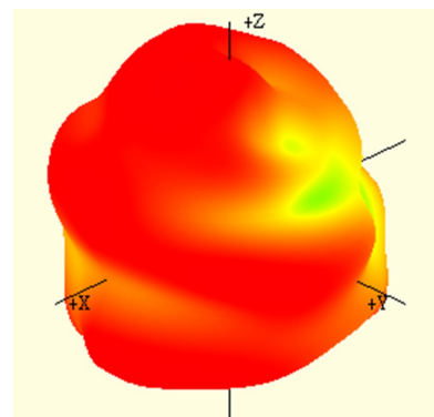
1602 MHz
