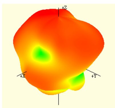
1176.45 MHz
