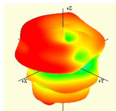
1602 MHz
