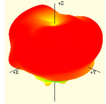
2690 MHz
