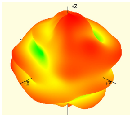
1561 MHz
