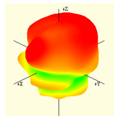
1602 MHz
