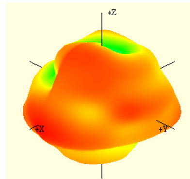
1238 MHz
