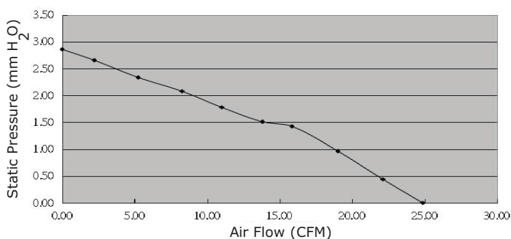
CFM-7010C-140-347
