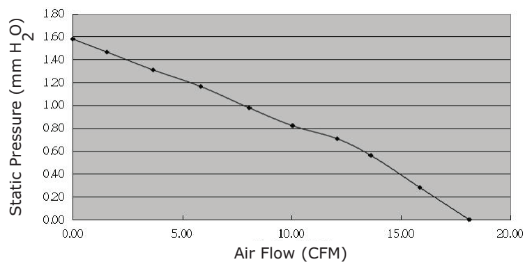
CFM-7015C-030-295
