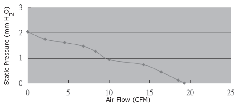
CFM-7015C-030-295
