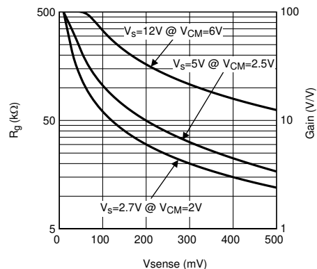
图 7-4. Allowed Gains for Range 2
