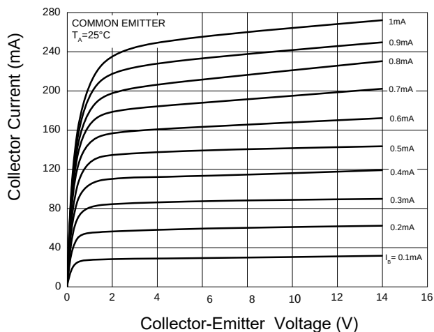
Fig. 1 - Static Characteristics
