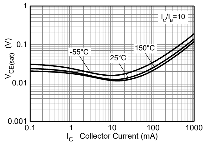
Fig.14 V_{CE(sat)} \text{ v } I_C (BC817-40)
