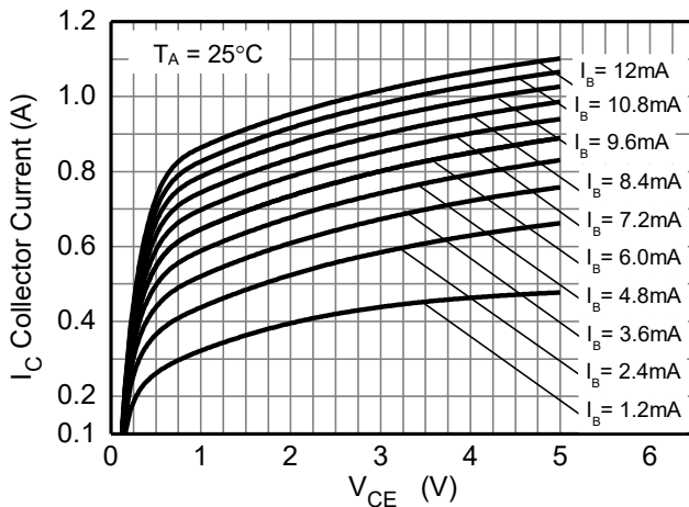
Fig.13 I_C \text{ v } V_{CE} (BC817-40)
