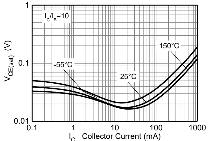
Fig.6 V_{CE(sat)} v I_C (BC817-16)
