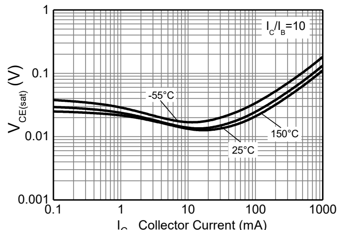
Fig.10 V_{CE(sat)} v I_C (BC817-25)
