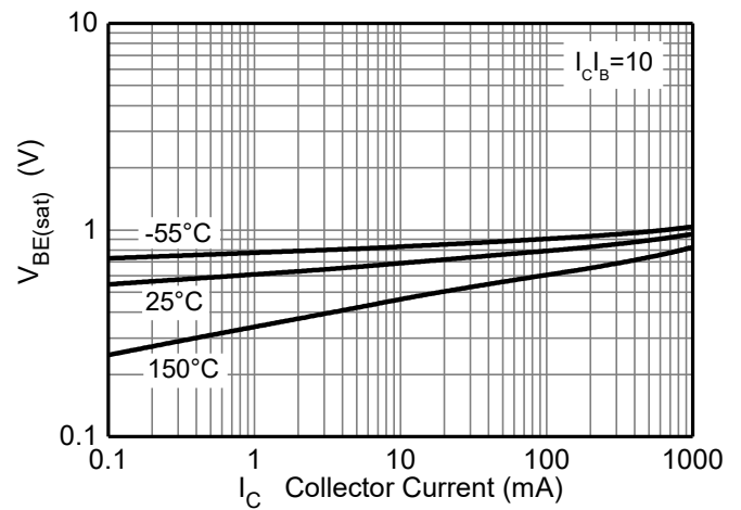
Fig.8 V_{BE(sat)} v I_C (BC817-16)
