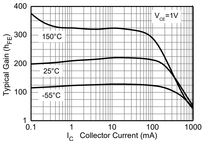
Fig.7 h_{FE} v I_C (BC817-16)
