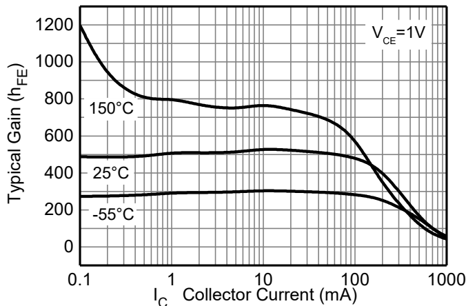
Fig.15 h_{FE} \text{ v } I_C (BC817-40)
