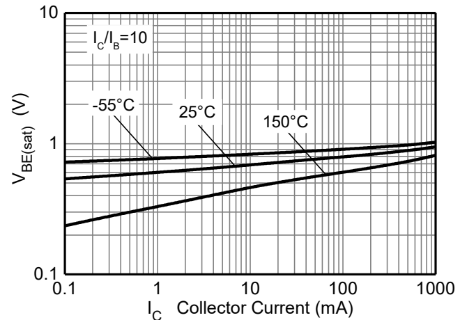
Fig.12 V_{BE(sat)} \text{ v } I_C (BC817-25)
