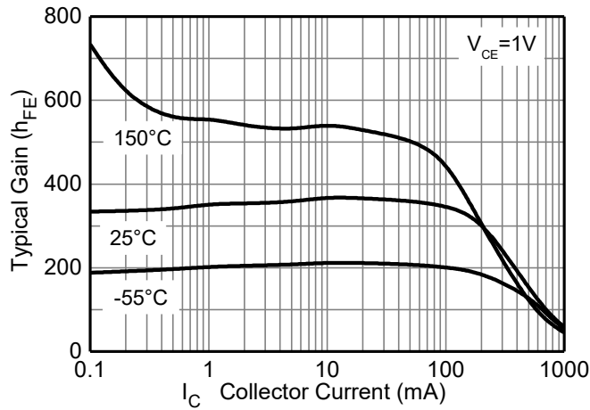
Fig.11 h_{FE} \text{ v } I_C (BC817-25)
