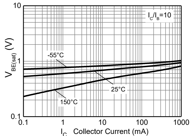
Fig.16 V_{BE(sat)} \text{ v } I_C (BC817-40)
