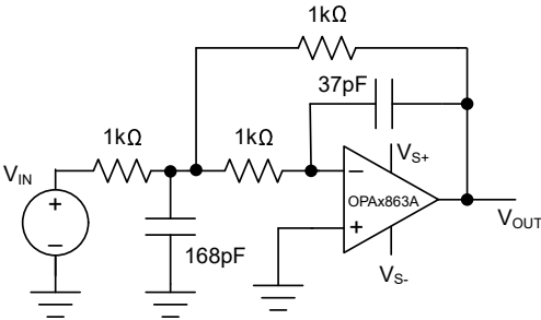
图 8-1. MFB Low-Pass Filter Circuit Using the OPAx863A
