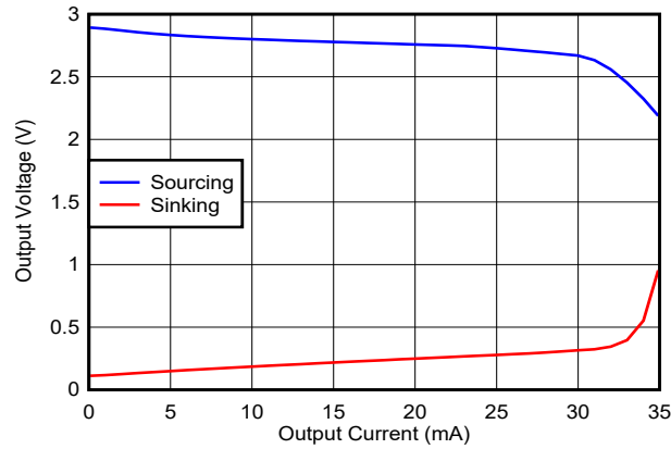
图 6-34. Output Voltage vs Load Current
