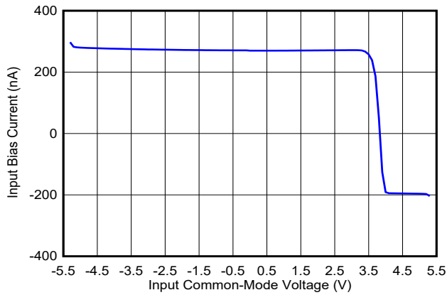
图 6-13. Input Bias Current vs Input Common-Mode Voltage
