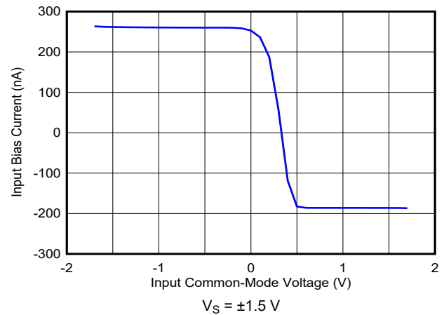
图 6-33. Input Bias Current vs Input Common-Mode Voltage
