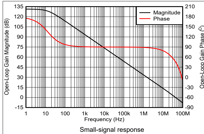
图 6-40. Open-Loop Gain and Phase vs Frequency
