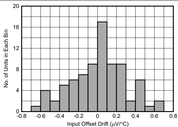
图 6-19. Input Offset Voltage Drift Distribution
