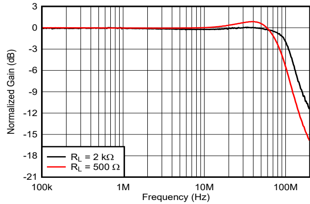
图 6-2. Small-Signal Frequency Response vs Output Load
