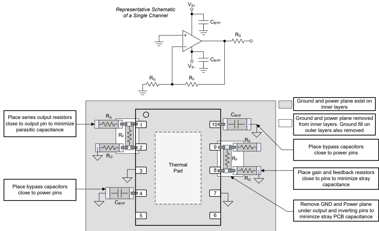
图 8-5. Layout Recommendation for Dual-Channel DSN Package
