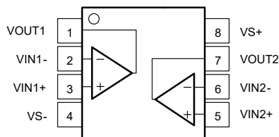
图 5-2. OPA2863A D Preview Package, 8-Pin SOIC and DGK Preview Package, 8-Pin VSSOP (Top View)
