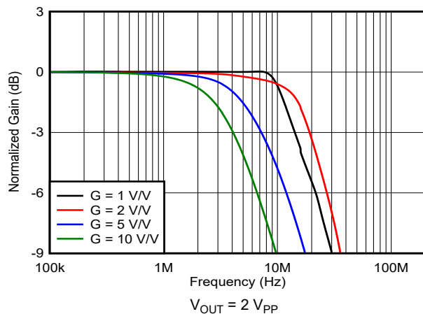
图 6-5. Large-Signal Frequency Response vs Gain
