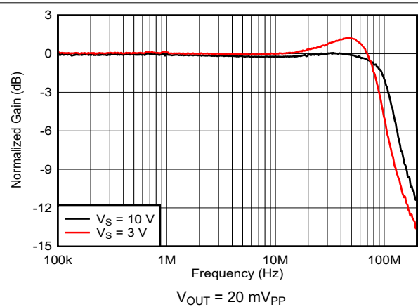
图 6-41. Frequency Response vs Supply Voltage
