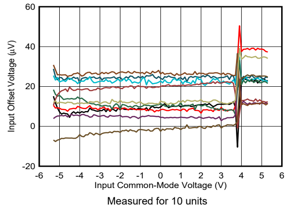
图 6-12. Input Offset Voltage vs Input Common-Mode Voltage
