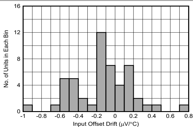
图 6-20. Input Offset Voltage Drift Distribution
