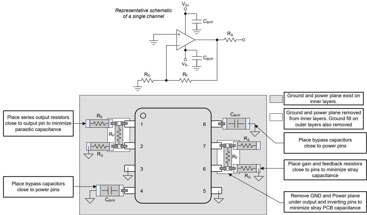
图 8-4. Layout Recommendation for Dual-Channel DGK Package
