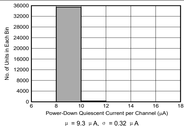
图 6-24. Power-Down Quiescent Current Distribution
