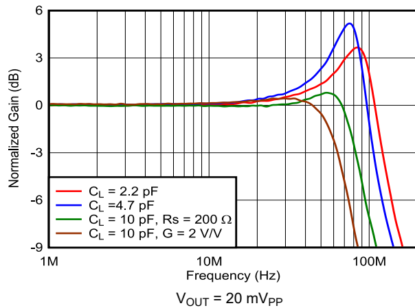
图 6-3. Frequency Response vs Load Capacitance
