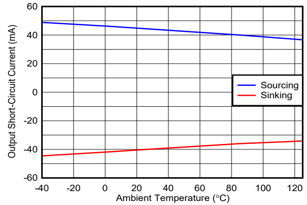
图 6-35. Output Short-Circuit Current vs Ambient Temperature
