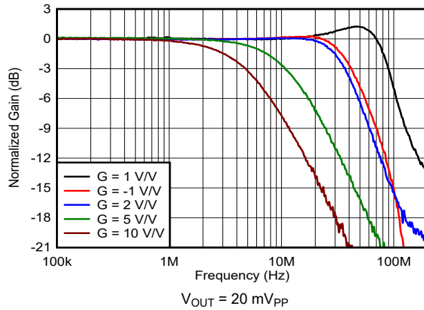
图 6-28. Small-Signal Frequency Response vs Gain
