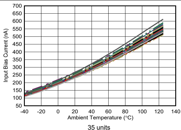
图 6-22. Input Bias Current vs Ambient Temperature
