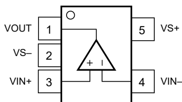
图 5-1. OPA863A DBV Package, 5-Pin SOT-23 (Top View)
