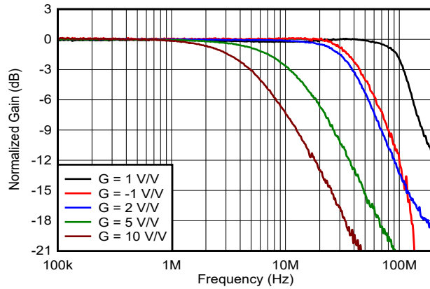
图 6-1. Small-Signal Frequency Response vs Gain
