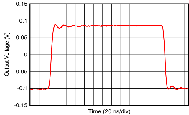
图 6-8. Small-Signal Transient Response
