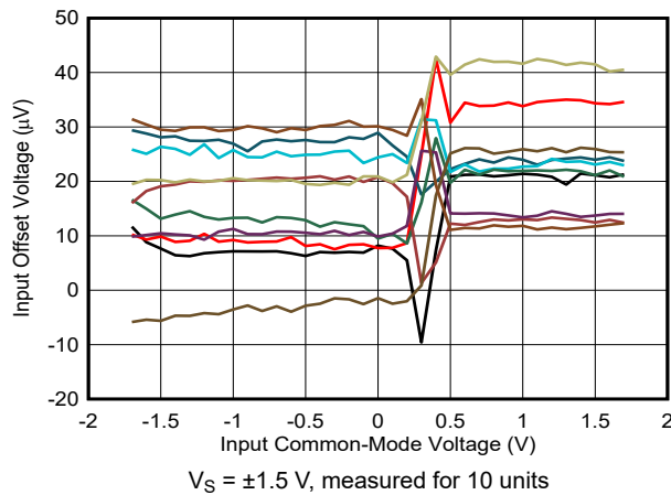
图 6-32. Input Offset Voltage vs Input Common-Mode Voltage
