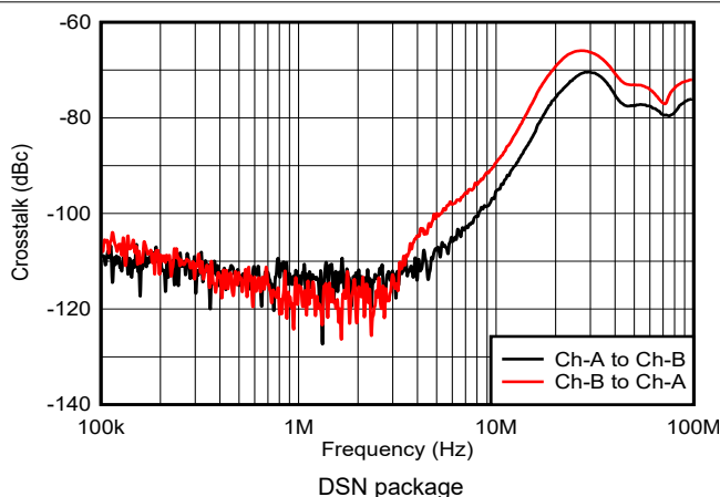
图 6-47. Crosstalk vs Frequency
