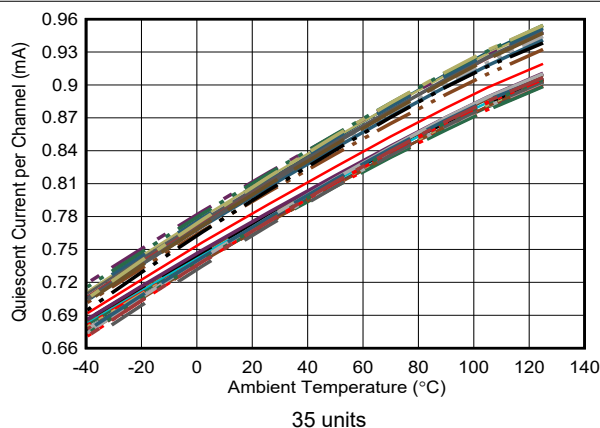
图 6-21. Quiescent Current vs Ambient Temperature
