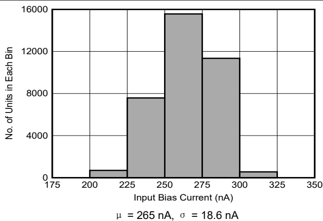
图 6-17. Input Bias Current Distribution
