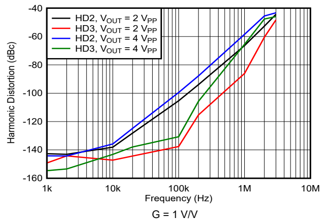
图 6-6. Harmonic Distortion vs Frequency
