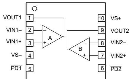
图 5-3. OPA2863A DSN Package, 10-Pin USON With Exposed Thermal Pad (Top View)
