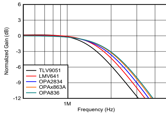
图 8-2. MFB Low-Pass Filter Frequency Response vs GBW
