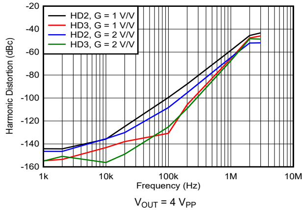
图 6-7. Harmonic Distortion vs Gain
