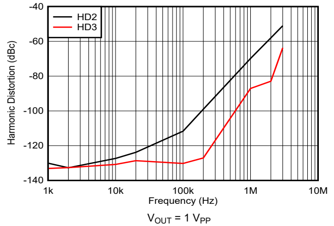
图 6-29. Harmonic Distortion vs Frequency
