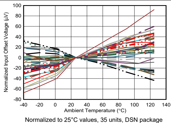
图 6-23. Input Offset Voltage vs Ambient Temperature
