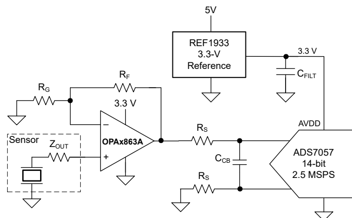
图 8-3. OPAx863A as a Precision SAR ADC Driver
