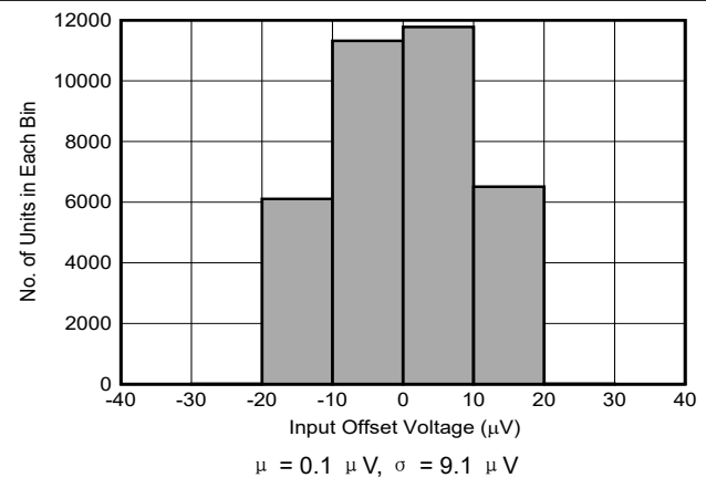
图 6-18. Input Offset Voltage Distribution
