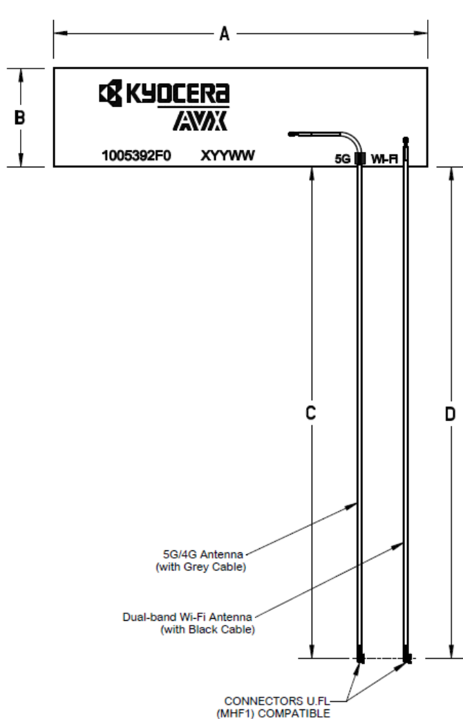
Top View
